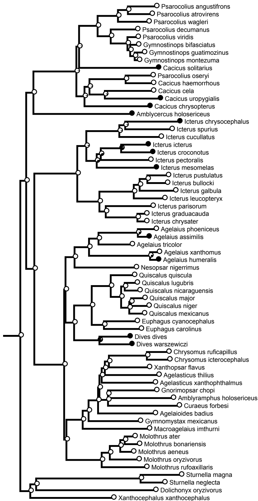
Supplementary Figure 1: Maximum-likelihood (Mk1) reconstruction of duetting in the New World blackbirds (Icteridae). Proportion of shading in circles represents the likelihood that duetting was present (black) or absent (white) at each node of the tree.
