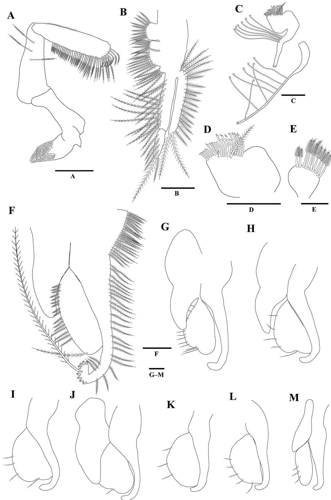
Fig. 3. Nebalia pseudotroncosoi n. sp., female holotype. A, mandibular palp; B, second maxilla; C, first maxilla; D, first maxilla, distal endite; E, first maxilla, proximal endite; F, thoracopod 1, showing setation; G, thoracopod 2; H, thoracopod 3; I, thoracopod 4; J, thoracopod 5; K, thoracopod 6; L, thoracopod 7; M, thoracopod 8. Scale bars = 0.2 mm (A-M).
