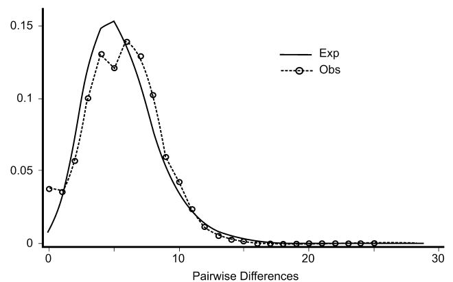
Fig. 8. Distribution curve from the mismatch analyses (raggedness index) showing observed (Obs) frequencies of pairwise differences among haplotypes and the expected (Exp) under the hypothesis of population expansion.
