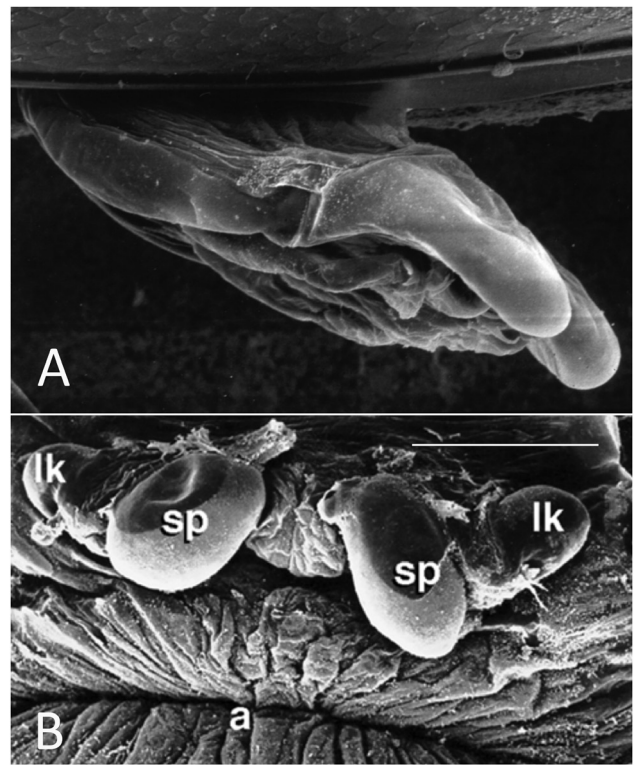
Figure 5. Copulatory (eighth) limbs. Male of undescribed H-Group species, right lateral view (A); female Enewton harveyi , ventral view (reprinted from Cohen & Morin, 2010 : fig. 24A) (B). Abbreviations: a, anus; lk, lateral knob; sp, spermatophore. Used with permission.
