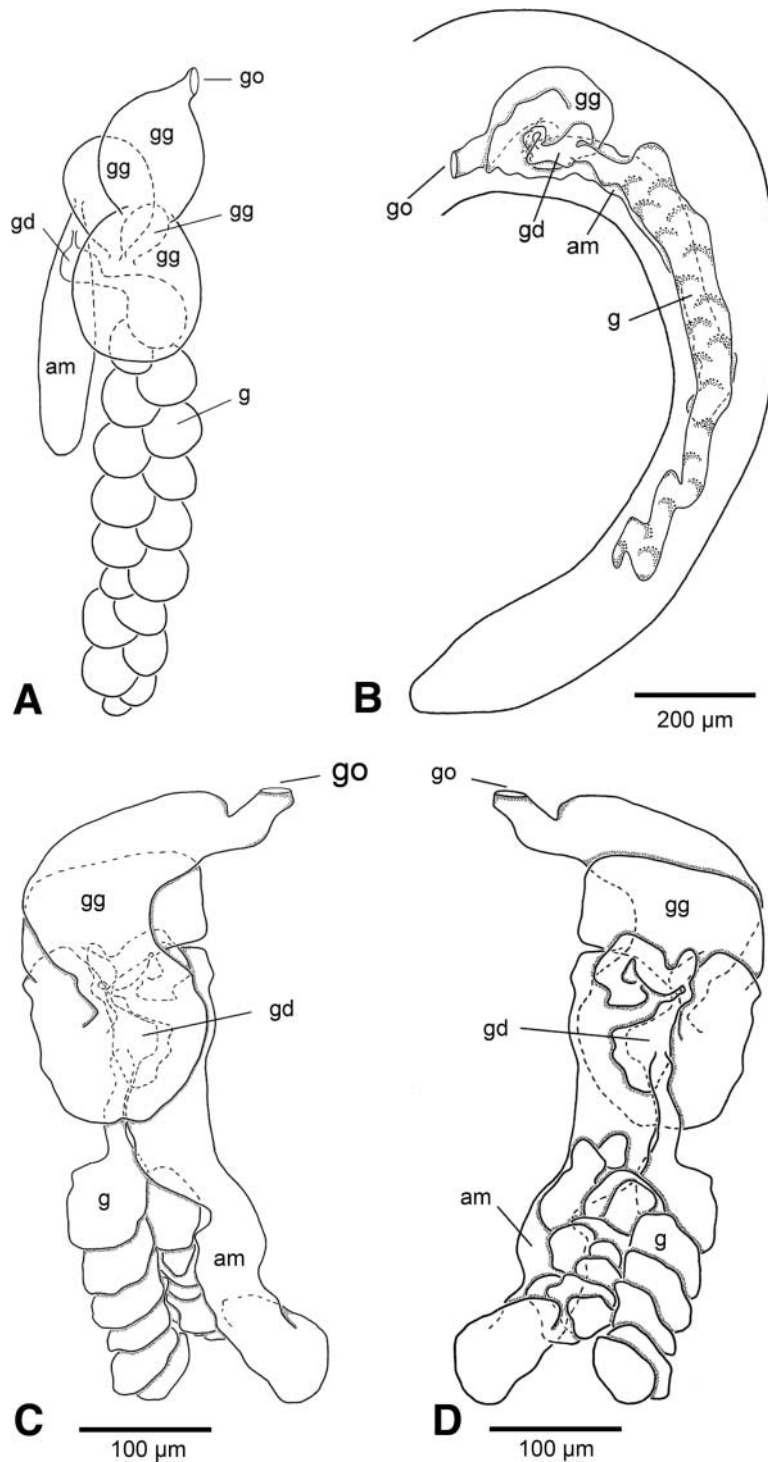
Figure 5. Reproductive system of Hedyloopsis ballantinei n. sp. A. Schematic drawing (dorsal view). B. Graphical reconstruction, lateral view. C. Graphical reconstruction, dorsal view. D. Graphical reconstruction, ventral view. Abbreviations: am, ampulla; g, gonad; gd, gonoduct; gg, genital gland; go, genital opening.
