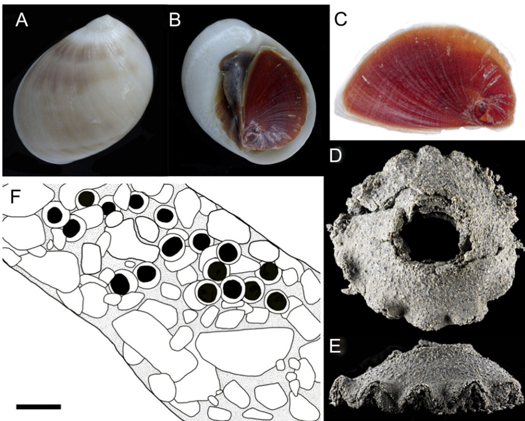
Figure 11. Mammilla melanostoma (Gmelin, 1791). A, B. Shell, Liufu (NMNS 003232-00039); SH 29 mm. C. Operculum, external surface; L 22 mm. D–F. Egg collar, Tongliang, Penghu, top, side view and cross-section; BD 89 mm; CH 18 mm. Scale bar F = 1 mm.
