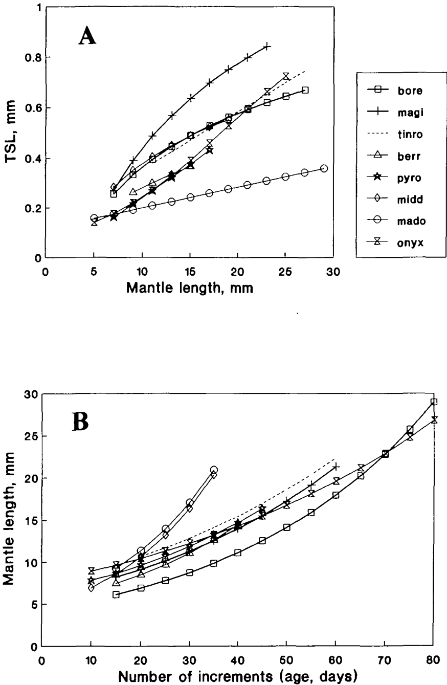
Fig. 17. Relative growth of total statolith length versus mantle length (A) and growth curves of mantle length (B) in gonatids from the western Bering Sea. bore, Gonatopsis borealis ; magi, Berryteuthis magister ; tinro, Eogonatus tinro ; berr, Gonatus berryi ; pyro, Gonatus pyros ; midd, Gonatus midden-dorffi ; mado, Gonatus madokai ; onyx, Gonatus onyx .
