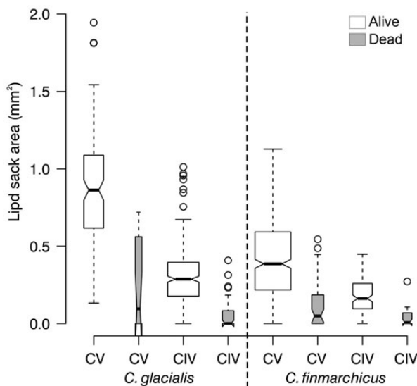
Fig. 3. Boxplot of the lipid sac area ( \text{mm}^2 ) of dead and alive copepodites stages IV and V of C. glacialis and C. finmarchicus in Rijpfjorden (whole water column, day and night pooled). Horizontal line shows the median. The bottom and top of the box show the 25 and 75 percentiles, respectively. Whiskers extend 1.5 times the inter-quartile range of the sample. Values outside this range are marked by circles. The boxes are drawn with widths proportional to the square-roots of the number of observations in the groups. Notches display the variability of the median between samples. The width of a notch is computed so that box plots whose notches do not overlap have different medians (Chambers et al. , 1983).
