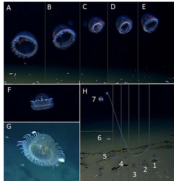
Fig. 7. The trachymedusa Crossota sp. from the Mariana Trench. (A–E) Close-up series of images of individual swimming passed the camera at 9066 m, each image is \sim 1.5 s apart. (F, G) The typical swimming position with tentacles pointed up and out. (H) A potential feeding event illustrated as a collage of the same event with image 1–7 being \sim 1 s apart, where 1–2 are descending to seafloor and repositioning tentacles down to make contact at 3, before ascending again in 4–7. Blue arrow indicates travel direction.
