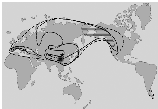
FIGURE 2. Distribution of Androsace (sect. Pseudoprimumula , solid line; sect. Chamaejasme , narrowly spaced dashed line; sect. Aizoidium , dashed-dotted line; sect. Andraspis , widely spaced dashed line; sect. aretia , dotted line) and the related genera Douglasia (horizontally hatched area), Pomatosace (star), and Vitaliana (vertically hatched area). The dark spot in East Asia indicates the center of species richness of Androsace (>35 species; see Meusel et al., 1978).
