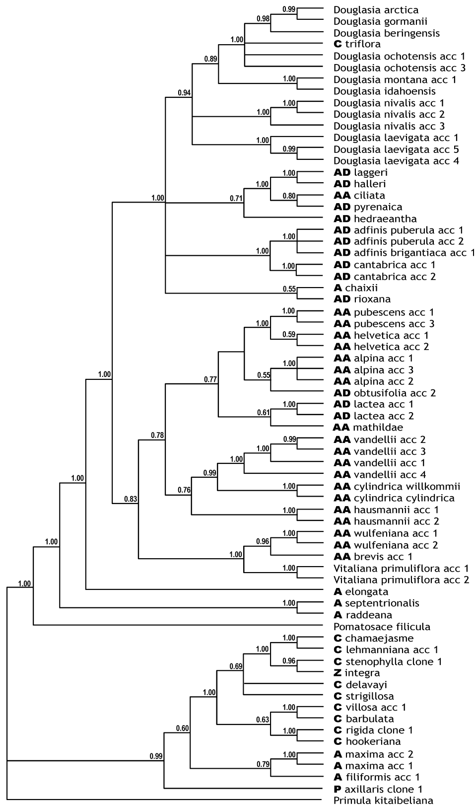
FIGURE 4. Phylogenetic relationships of Androsace and related genera inferred from Bayesian analysis of combined nuclear ITS and plastid trnLF regions (50% majority-rule consensus tree). Numbers above branches nodes represent posterior probability values \geq 0.5 . Abbreviations as in Figure 3.
