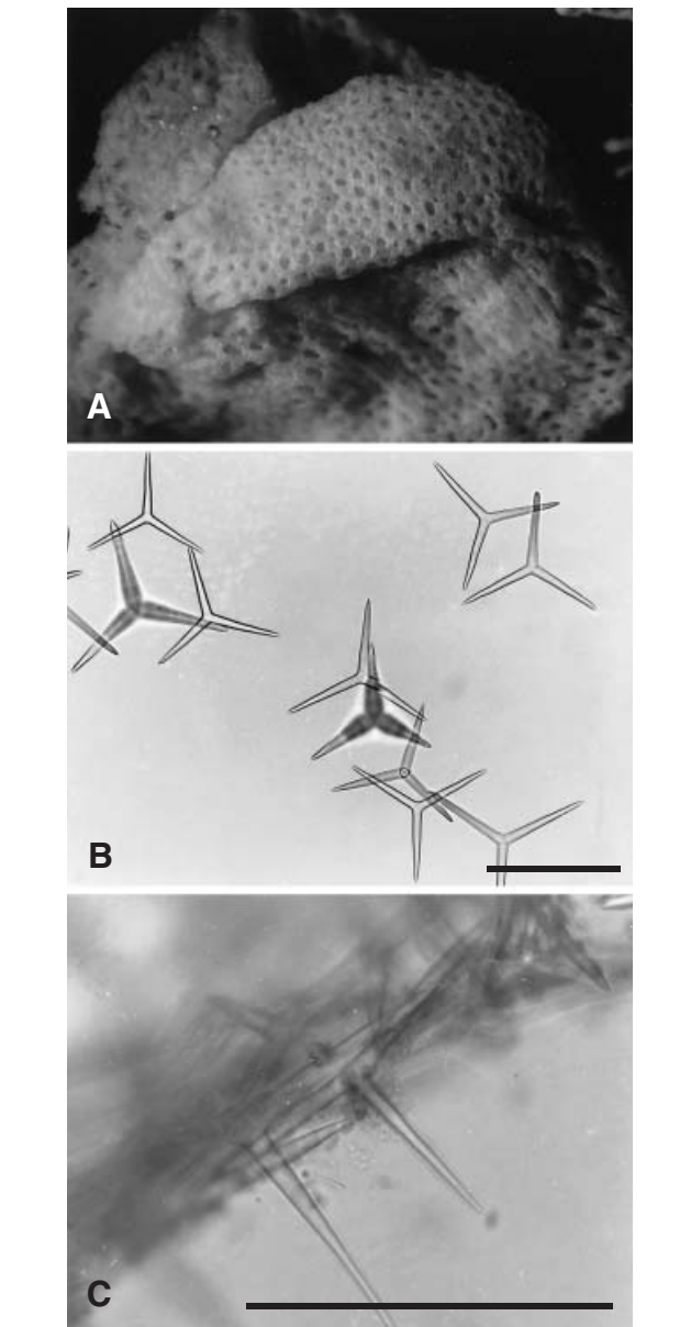
Figure 3. Clathrina aspina . A, photograph of the holotype ( \times 10 ). B, triactines, tetractines and tripods. C, apical actine of the tetractines. Scale bar = 100 µm.
