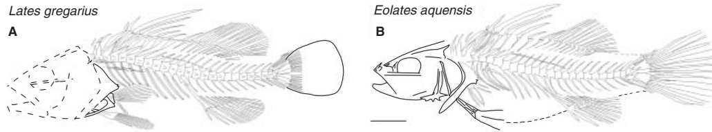
Figure 26. General view of the postcranial skeleton, in lateral view, of A, † Lates gregarius (from Bannikov, 1992; modified), and B, † Eolates aquensis (reconstruction mostly from NHM P3912). Scale bar = 10 mm.
