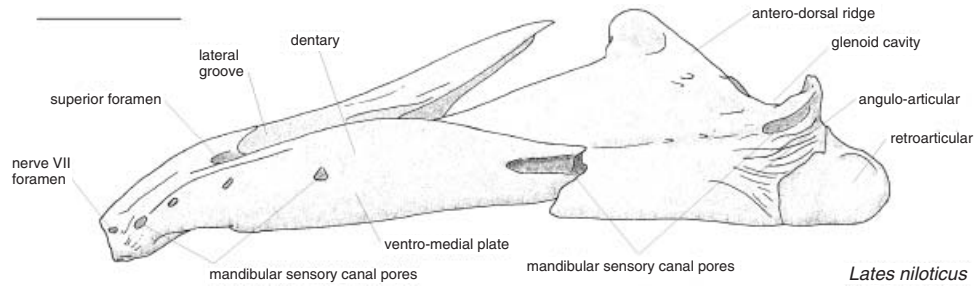
Figure 23. Right (reversed) lower jaw of Lates niloticus (NHM 28.228 [4]), in latero-ventral view. Scale bar = 10 mm.
