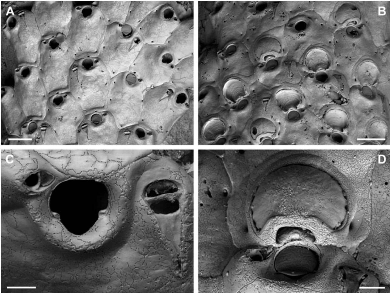
Figure 4. Buffonellaria ritae sp. nov.: holotype, NHM 2007.5.18.6, Madeira, off Santa Cruz. A, general aspect of autozoecia; scale bar, 200 \mu m. B, ovicellate zoecia; scale bar, 200 \mu m. C, close-up of orifice and oral avicularia; scale bar, 50 \mu m. D, close-up of oecium; scale bar, 50 \mu m.
