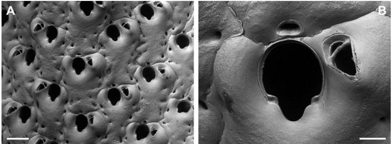
Figure 10. Buffonellaria sp. 1: NHM 2007.5.18.12, off Toulon, Mediterranean Sea. A, general aspect of autozoecia; scale bar, 200 \mu\text{m} . B, Close-up of orifice; scale bar, 50 \mu\text{m} .
