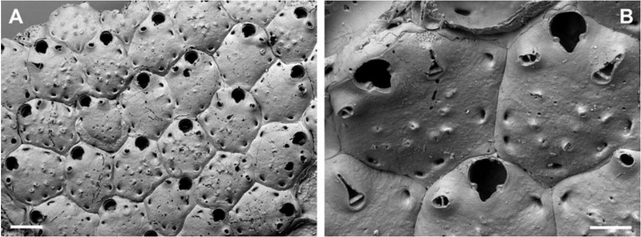
Figure 15. Buffonellaria sp. 2: SMF 3015, off Sierra Leone. A, general aspect; scale bar, 200 \mu m. B, Close-up of auto-zoecia; scale bar, 100 \mu m.
