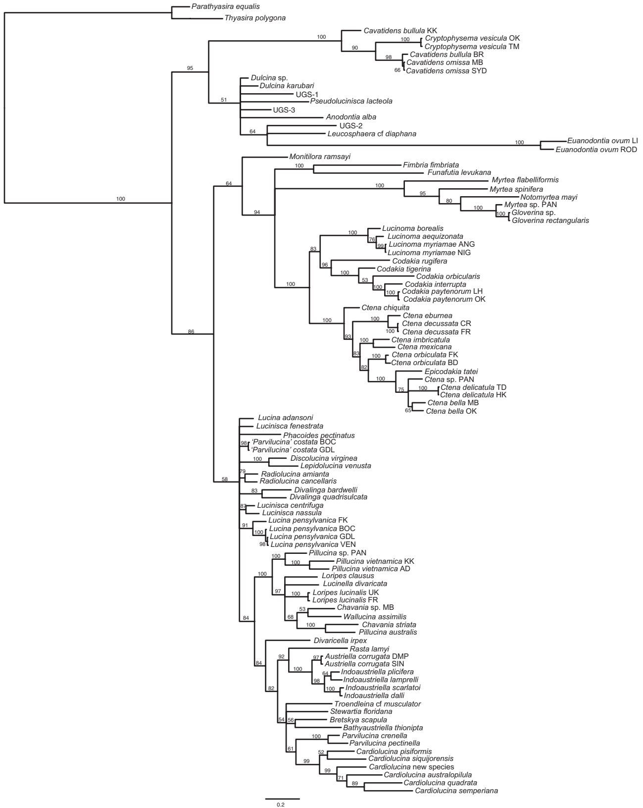
Figure 3. Molecular phylogeny of the Lucinidae based on the single gene analysis of cytochrome b produced by Bayesian analysis using MRBAYES. Support values are Bayesian posterior probabilities (%). Details of taxa are given in Table 1.
