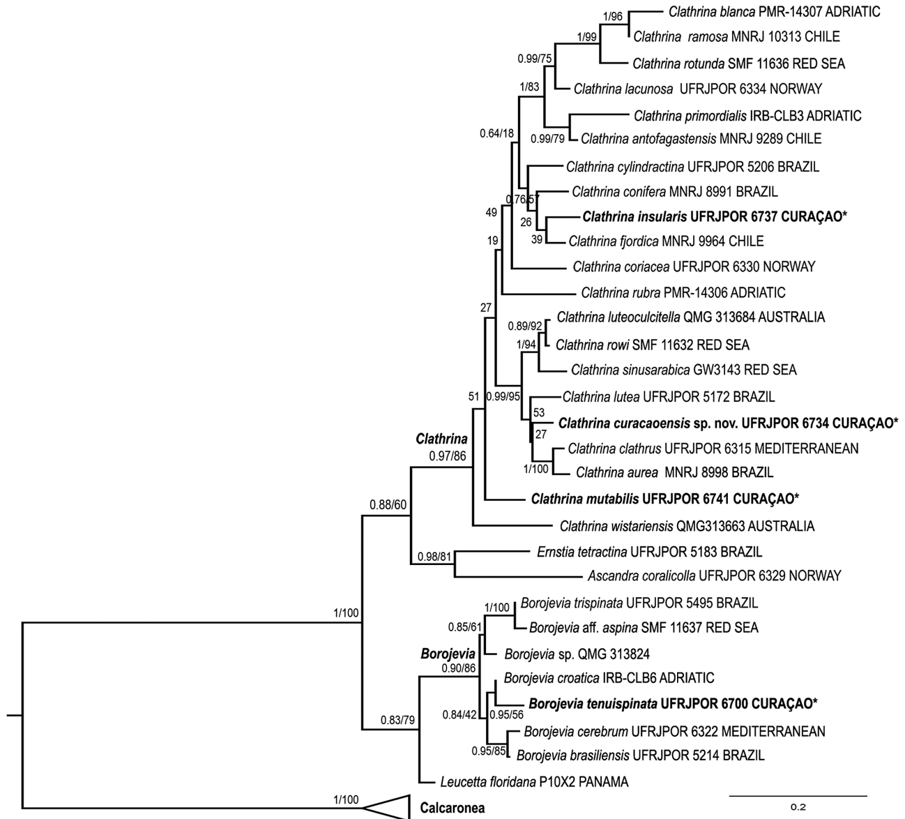
Figure 5. Maximum likelihood phylogenetic tree inferred from the C-LSU sequences of the Calcarea species. Posterior probabilities and bootstrap values are given on the branches (pp/bootstrap). *Sequences generated in this study.
