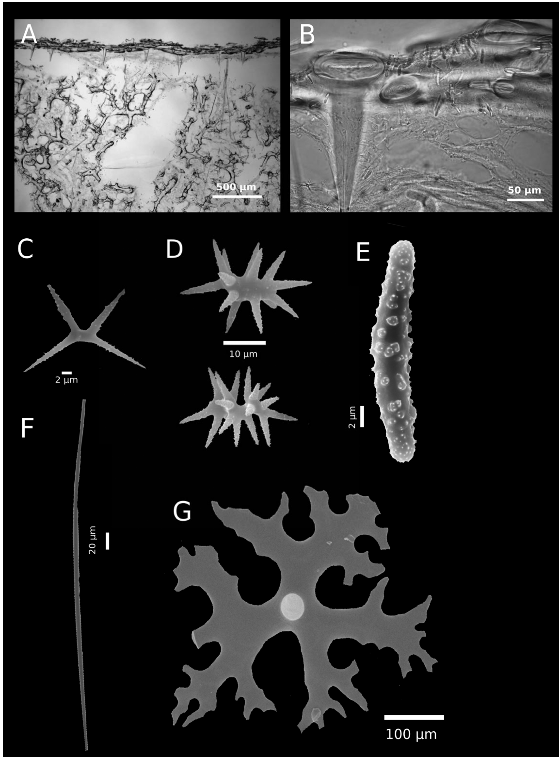
Figure 9. Racodiscula radixa sp. nov. Harbor Branch Oceanographic Museum (HBOM) 003:02006. A, B, thick sections showing phyllotrias with acanthorhabds on top (A) and in between (B), forming a thick crust on the surface. C, metaster. D, spiraster. E, acanthorhabds. F, tylostyles. G, ectosomal phyllotriaene.
