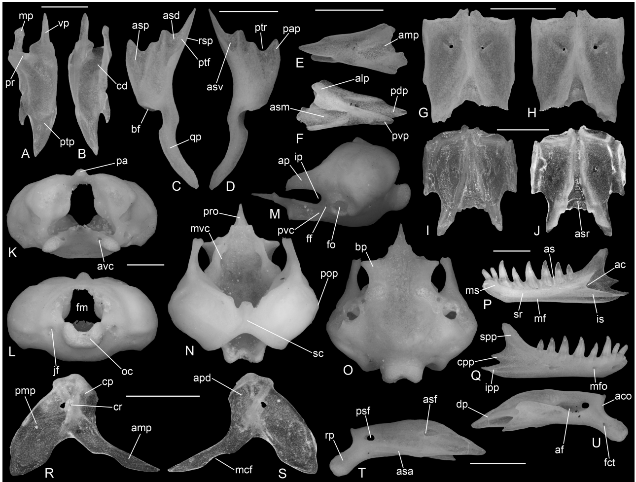
Figure 10. A–B, Blanus strauchi (MDHC 287), left palatine in dorsal (A) and ventral (B) views. C–D, B. strauchi (MDHC 287), right pterygoid in dorsal (C) and ventral (D) views. E–F, B. strauchi (MDHC 288), left ectopterygoid in medial (E) and lateral (F) views. G–H, Blanus vandellii (MDHC 156), tabulosphenoid in dorsal (G) and ventral (H) views (the left posterior process is broken). I–J, B. strauchi (MDHC 287), tabulosphenoid in dorsal (I) and ventral (J) views. K–O, B. strauchi (MDHC 287), otooccipital region in anterior (K), posterior (L), left lateral (M), dorsal (N) and ventral (O) views. P–Q, B. strauchi (MDHC 287), right dentary in medial (P) and lateral (Q) views. R–S, B. strauchi (MDHC 287), left coronoid in medial (R) and lateral (S) views. T–U, B. vandellii (MDHC 156), right compound bone in lateral (T) and medial (U) views. Abbreviations: ac, alveolar canal; aco, articular condyle; af, adductor fossa; alp, anterolateral process; amp, anteromedial process; ap, alar process; apd, articular surface with the superior posterior process of the dentary; as, alveolar shelf; asa, articular surface with the angular; asd, articular surface with the posterodorsal process of the ectopterygoid; asf, anterior surangular foramen; asm, articular surface with the maxilla; asp, articular surface with the palatine; asr, articular surface with the parasphenoid rostrum of the sphenoid; asv, articular surface with the posteroventral process of the ectopterygoid; avc, anterior opening of the Vidian canal; bf, basiptyergoid fossa; bp, basiptyergoid process; cd, choanal duct; cp, coronoid process; cpp, central posterior process; cr, coronoid ridge; dp, dentary process; fct, foramen for the chorda tympani; ff, facial foramen; fm, foramen magnum; fo, fenestra ovalis; ip, incisura prootica; ipp, inferior posterior process; is, intramandibular septum; jf, jugular foramen (concavity of the vagus foramen); mcf, notch of the mandibular central foramen; mf, Meckelian fossa; mfo, mental foramen; mp, maxillary process; ms, mandibular symphysis; mvc, medial opening of the Vidian canal; oc, occipital condyle; pa, processus ascendens; pap, palatine process; pdp, posterodorsal process; pmp, posteromedial process; pop, paroccipital process; pr, palatine ridge; pro, parasphenoid rostrum; psf, posterior surangular foramen; ptf, pterygoid flange; ptp, pterygoid process; ptr, pterygoid recess; pvc, posterolateral opening of the Vidian canal; pvp, posteroventral process; qp, quadrate process; rp, retroarticular process; rsp, ridge for the insertion of the superficial pseudotemporal muscle; sc, supraoccipital crest; spp, superior posterior process; sr, subdental ridge; vp, vomerine process. Scale bars: 1 mm.
