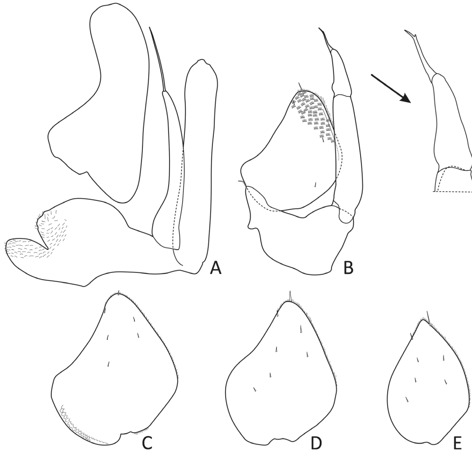
Figure 25. Alpiniscus (Illyrionethes) hirci Bedek & Taiti sp. nov. Paratype ♂ CBSSC IT2389, from Bukovac: A, genital papilla and pleopod 1; B, pleopod 2 with enlargement (arrow) of endopod distal article; C, pleopod 3 exopod; D, pleopod 4 exopod; E, pleopod 5 exopod.
