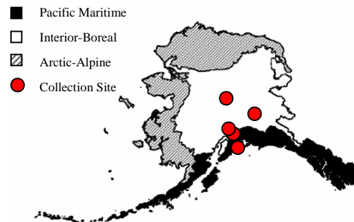
Distribution of yellow alfalfa in Alaska
