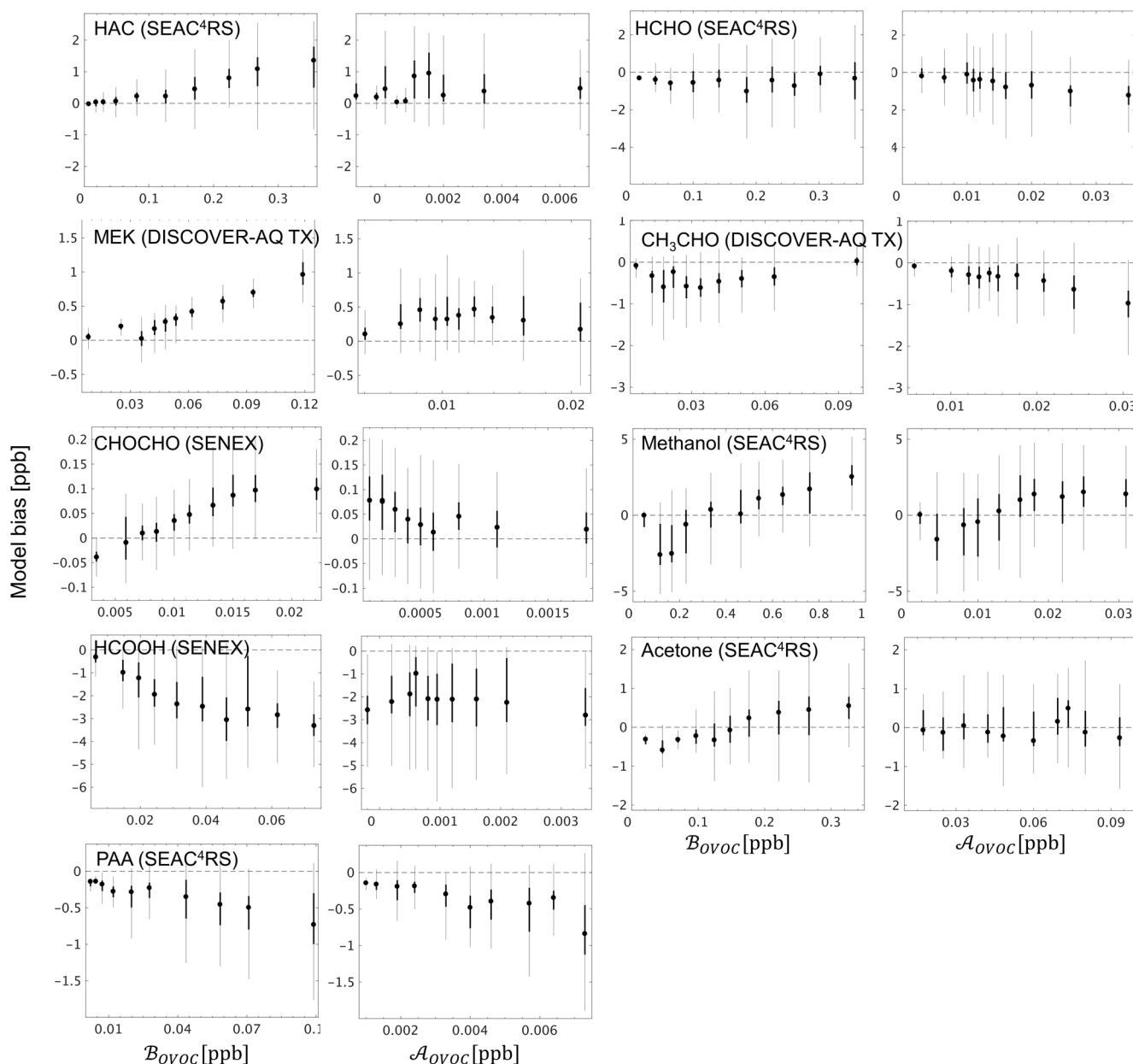
Figure 10. GEOS-Chem model bias for select OVOCs in the boundary layer (< 1 km here), binned according to the contribution from biogenic ( B_{OVOC} ) and anthropogenic ( A_{OVOC} ) sources to the overall abundance. B_{OVOC} and A_{OVOC} represent the integrated influence of primary + secondary biogenic and anthropogenic sources (respectively) for a given OVOC along the aircraft flight track based on the model simulation, as described in the text. The 10 plotted bins each represent an equal number of data points for a given OVOC, with the box plots indicating the corresponding median (filled circle), interquartile range (thick line), and 99 % confidence interval (thin line).
