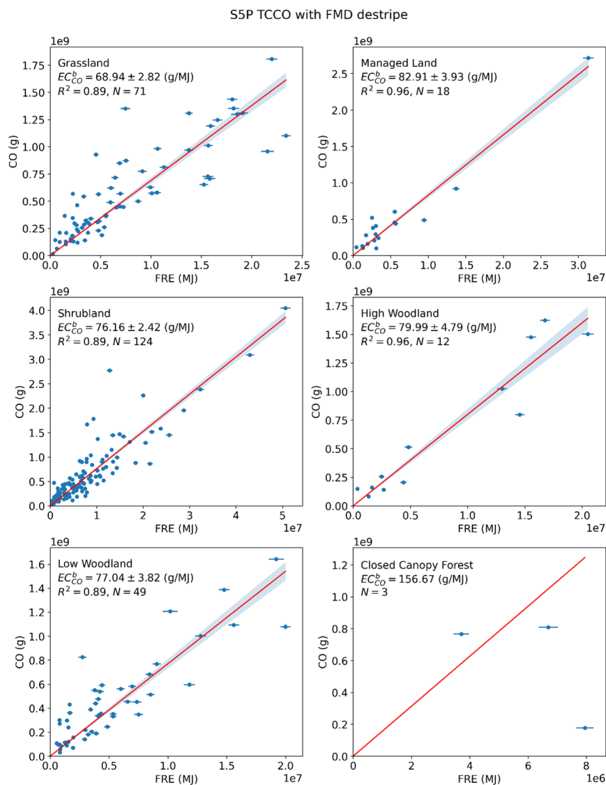
Figure A1. CO emissions coefficients ( EC_{CO}^b ) derived with FMD applied to the S5P TCCO data.
