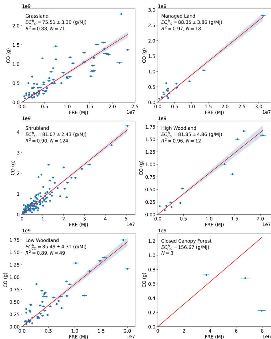
Figure 2. Carbon monoxide smoke emission coefficients ( EC_{CO}^b ; in g\ MJ^{-1} ) derived from match-up fires burning across the six fire-affected biomes shown mapped in Fig. 8b across Southern Hemisphere Africa (note that the match-up fires here come from both African hemispheres). Each EC_{CO}^b is derived from the slope of an ordinary least-squares (OLS) regression between the fire-emitted CO calculated from Sentinel-5P total column CO (TCCO) observations and the fire's matching FRE. The shaded grey area indicates the error of each slope. Error bars represent the uncertainty in both the FRE and total plume CO calculated from the uncertainty measures of the FRP-PIXEL product and the SSP TCCO product respectively. Closed-canopy forest had insufficient match-up fires identified, and so EC_{CO}^b for this biome was derived using the FEER-equivalent procedure detailed in Sect. 2.3 and in Nguyen and Wooster (2020). Data points from the three match-up fires that were identified in closed-canopy forest are included in the plot.
