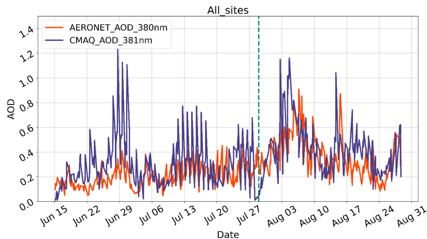
Figure D1. Hourly AOD averaged over all six AERONET sites, both from the CMAQ simulations and AERONET observations. A vertical dotted line on 29 July indicates the start of the second simulation.
