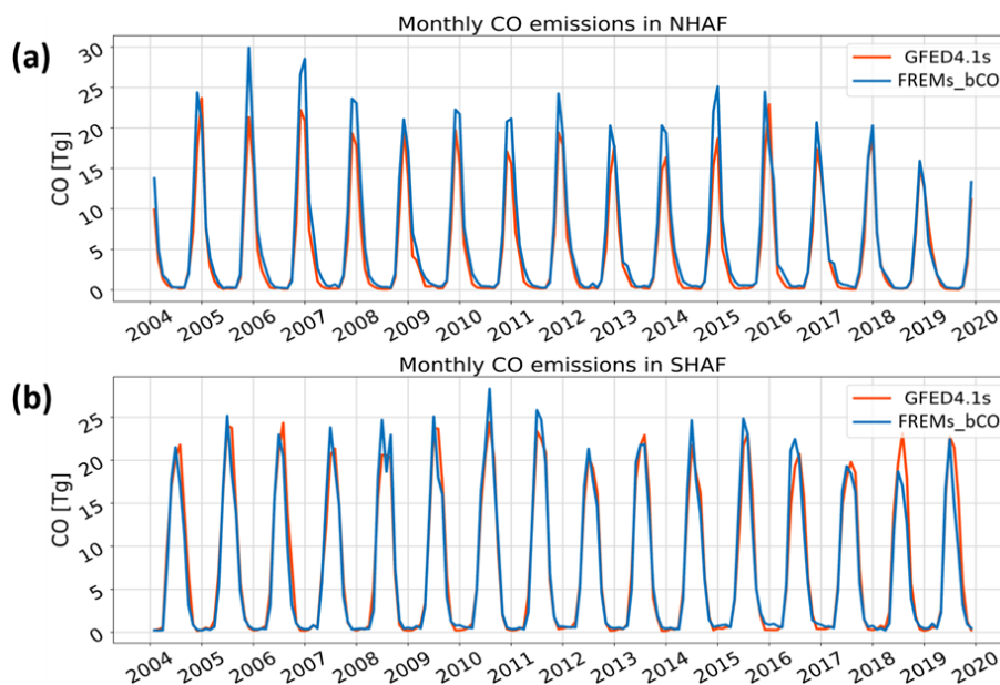
Figure 3. Monthly landscape fire CO emissions over a 16-year period for (a) Northern and (b) Southern Hemisphere Africa, as derived in FREMs_bCO and GFED4.1s, both with their respective small fire correction applied (“s” indicates its application).
