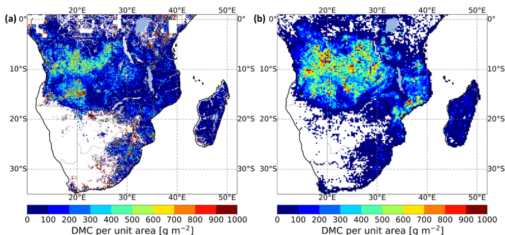
Figure 6. Dry matter consumed (DMC) per unit area, mapped across Southern Hemisphere Africa for 2019. (a) As calculated in 0.1^\circ grid cell resolution by dividing the FREMs_bCO CO values (with SF correction) by the 20 m FireCCISFD burned area product generated from Sentinel-2 MSI observations and (b) as reported in GFED4.1s at 0.25^\circ grid cell resolution.
