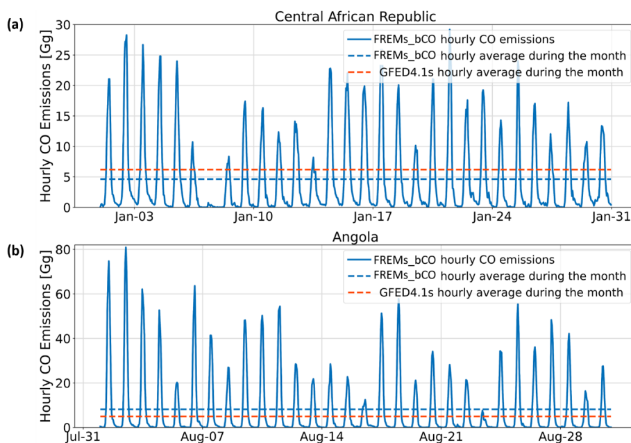
Figure 4. Hourly FREMs_bCO emissions from landscape fires burning over a month-long period in 2012 during the peak fire season of (a) the Central African Republic and (b) Angola. The monthly mean of this emission rate is also shown, along with that from GFEDv4.1s.
