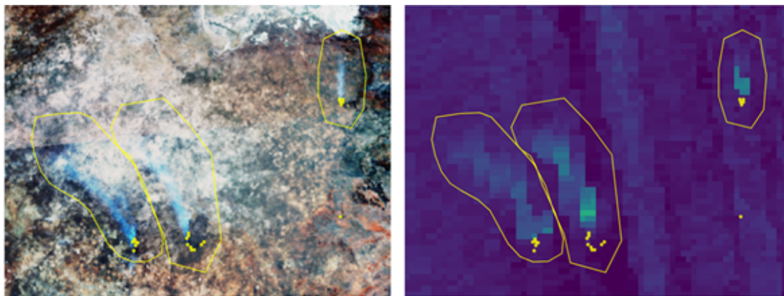
Figure 1. Example data of match-up fires used to develop the C_e^{CO} smoke emissions coefficients presented in Fig. 2. (a) VIIRS RGB image of three landscape fire smoke plumes, along with (b) the corresponding image of Sentinel-5P derived total column CO (TCCO). In both images, the AF pixel detections taken from the Meteosat FRP-PIXEL product are superimposed (yellow points), along with the bounding polygons used to delineate the fire plumes. Satellite data are from 11:24 and 11:30 UTC, respectively, on 9 September over an area in northern Botswana.
