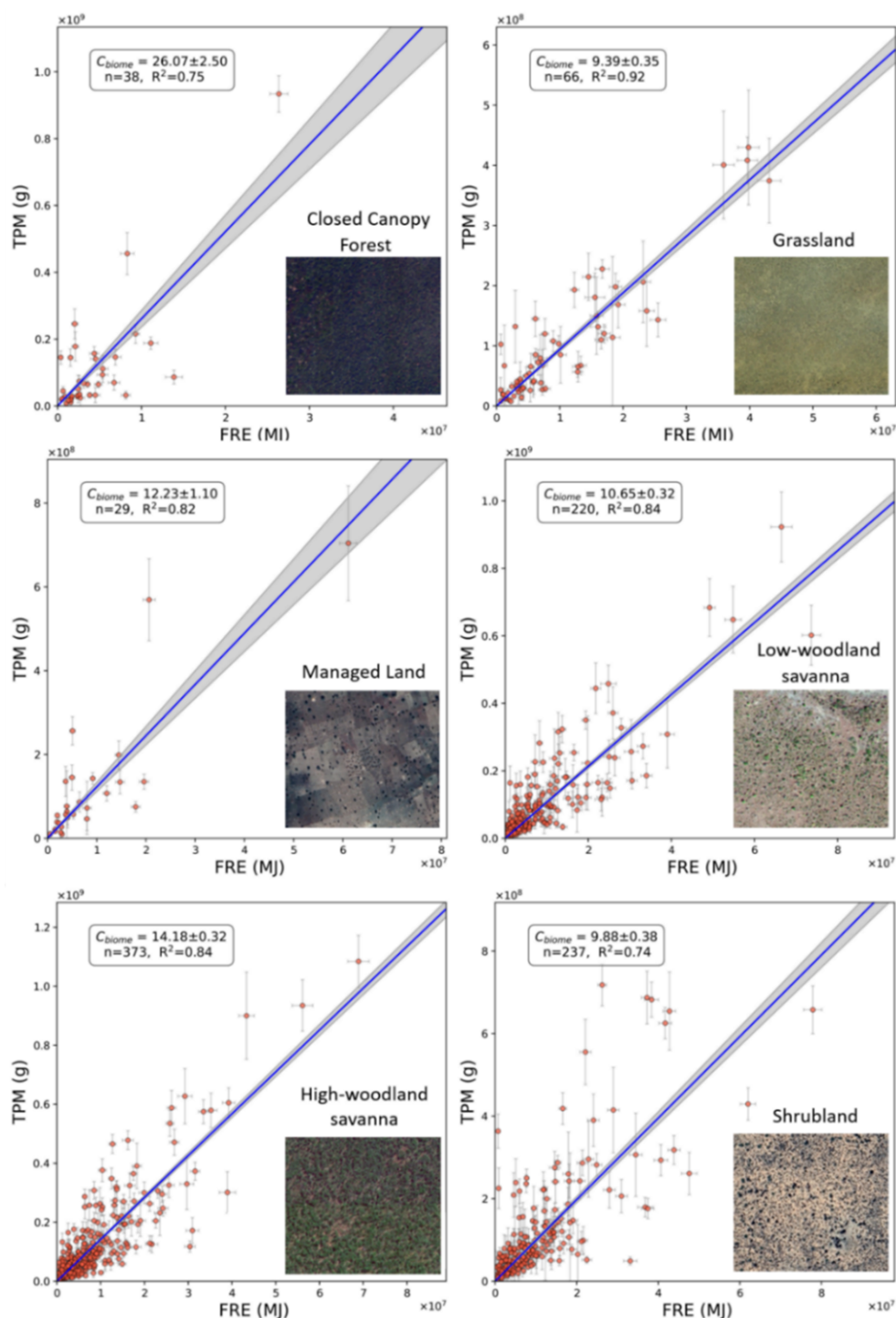
Figure B1. TPM smoke emission coefficients ( C_{\text{C}}^{\text{TPM}} ; in g MJ -1 ) for the six African fire-affected biomes defined in the main text, each derived from the slope of an ordinary least-squares (OLS) regression between data of fire-emitted total particulate matter (TPM) and matching fire radiative energy (FRE). The grey shaded area defines the 95 % probability prediction interval of the OLS-derived slope. Each scatter plot is accompanied by an illustrative insert that depicts the typical land cover for the biome as seen in © Google Earth (example locations are closed-canopy forest 10.359° S, 19.086° E; grassland 21.180° S, 19.560° E; managed land 10.495° N, 7.586° E; low-woodland savanna 7.085° N, 27.095° E; high-woodland savanna 12.523° S, 23.323° E; and shrubland 23.055° N, 22.242° E).
