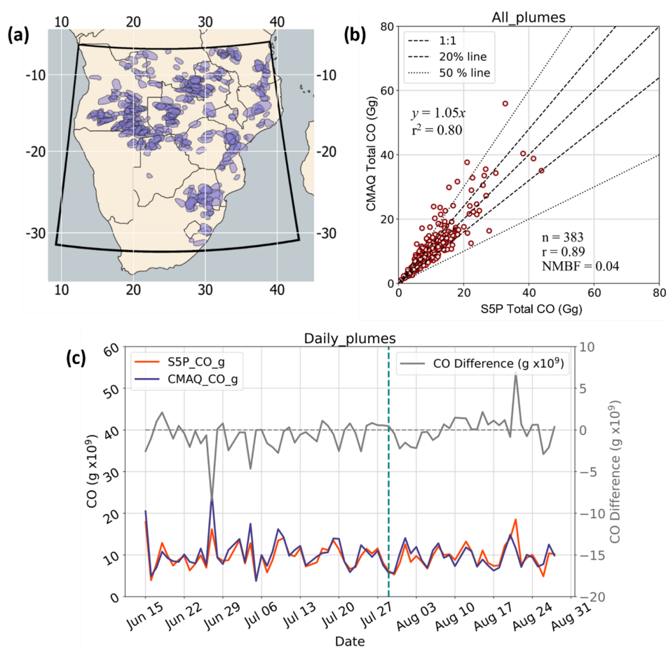
Figure 11. Evaluation of FREM-derived CO emissions based on WRF-CMAQ modelling. (a) Model domain and the bounding polygons of 383 plumes identified in the S5P TCCO product between 15 June and 29 August 2019 used in the evaluation. (b) Relationship between modelled and observed total in-plume CO for the individual smoke plumes identified in (a) . Pearson's correlation and NMBF of the dataset are shown, along with dotted lines indicating the 1 : 1, \pm 20\% and \pm 50\% relationships. The NMBF of 0.04 indicates a 4 % mean overestimation by the model compared to the observations. (c) Summed total CO from all plumes observed on each day of the simulation as determined by CMAQ (purple) and S5P (red), with their difference represented by the grey line (right-hand-side y axis). The vertical dotted line on 29 July indicates the start of the second simulation period (see main text).
