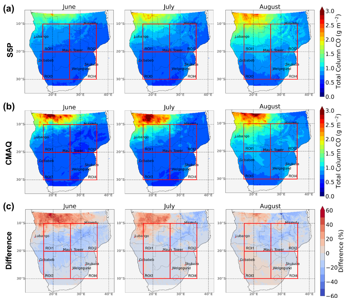
Figure 9. Mapped mean monthly total column carbon monoxide (TCCO) between 15 June and 29 August 2019, as determined by (a) S5P observations typically observed between 12:00 and 14:00 UTC and (b) CMAQ-averaged model TCCO output between 12:00 and 14:00 UTC; the model is fed with the FREMs_bCO emissions inventory developed herein. Their percentage difference is shown in (c).
