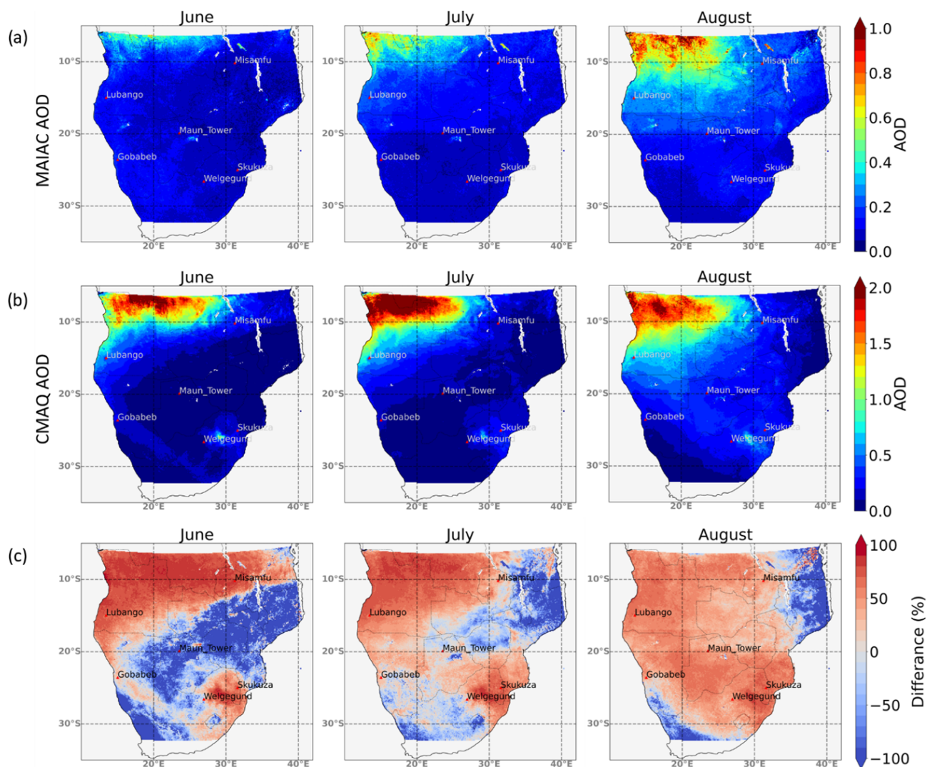
Figure D2. Mapped mean monthly AOD at 550 nm from (a) the MAIAC satellite product and (b) CMAQ simulations (note the colour scale differences between a and b) during the simulation period from 15 June to 29 August 2019. Panel (c) shows the percentage difference between MAIAC and CMAQ AOD.
