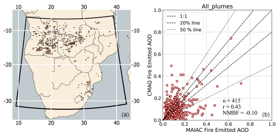
Figure D3. Location of smoke plumes identified in the MAIAC 1 km AOD product between 15 June and 29 August 2019 and the bounding polygons used to define the area over these plumes (a). Relationship between fire-emitted CMAQ AOD and observed fire-emitted MAIAC AOD in these plumes (b). Pearson's correlation and NMBF of the dataset are shown, along with dotted lines indicating the 1 : 1, 20 % and 50 % lines.
