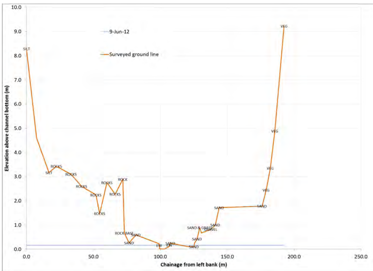
FIGURE 4.26: CROSS-SECTION SURVEYED FOR THE MALAPATI SITE SHOWING THE WATER LEVEL THAT WAS OBSERVED ON 9 JUNE 2012, EW = SURVEYED EDGE OF WATER
