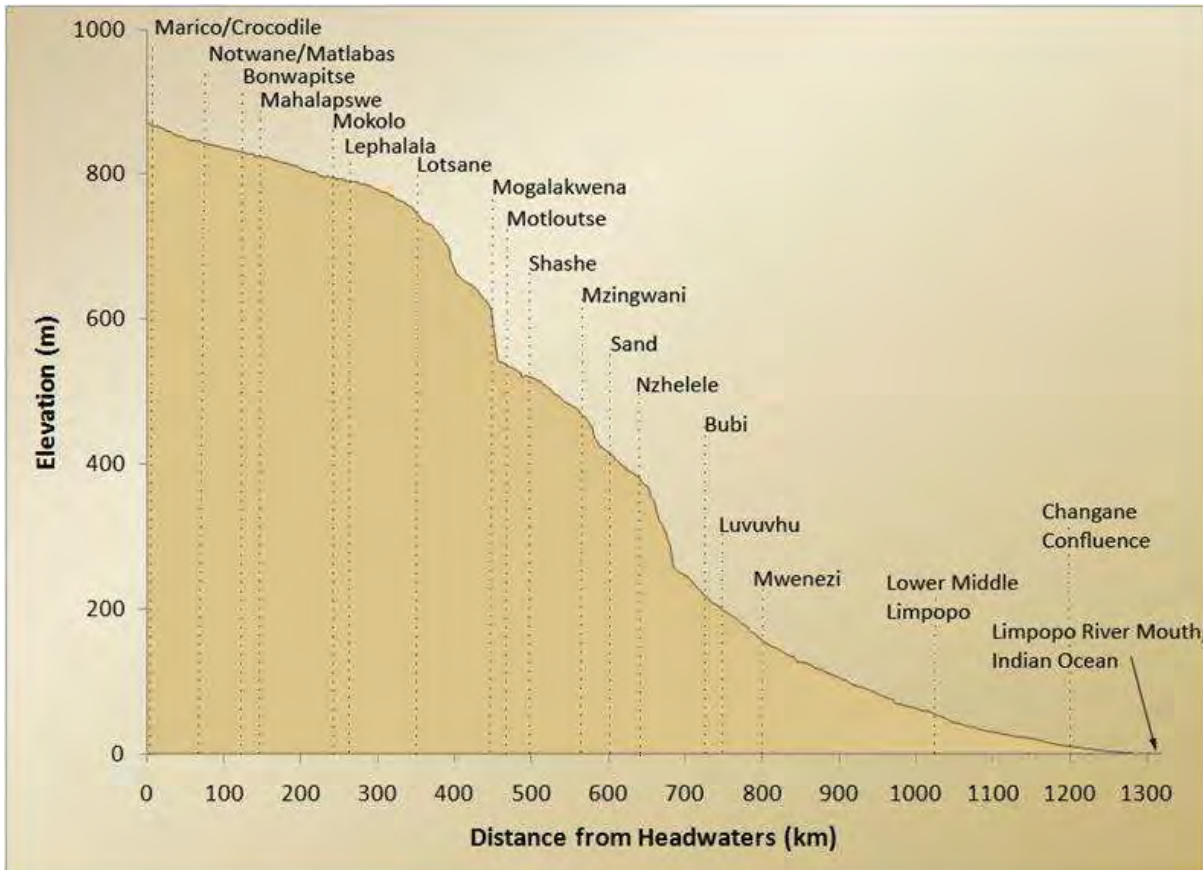
FIGURE 4.8: LONGITUDINAL PROFILE OF THE LIMPOPO RIVER AND THE LOCATIONS OF TRIBUTARIES JOINING THE MAIN STEM (FROM THE LIMPOPO RIVER AWARENESS KIT, 2020)
