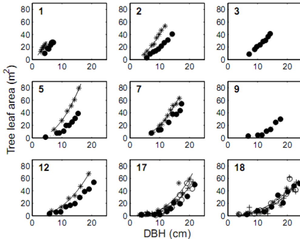
Figure 1: Tree leaf area as a function of DBH for the nine stands of destructive LAI measurements (numbers relate to stand number in Table 1), for the 2008 wet season (stars) and 2008 dry season (closed circles). For stands 17 and 18, there are also measurements in the 2007 dry season (open circles), and 2009 wet season (cross). All power adjustments on clonal stands (see Appendix A Eq. A1 and Eq. A2) have a R^2 > 0.92 and Root Mean Square Error < 2.96 \text{ m}^2 . On the Itatinga stands (17 and 18), all R^2 > 0.78 and \text{RMSE} < 10 \text{ m}^2 .
