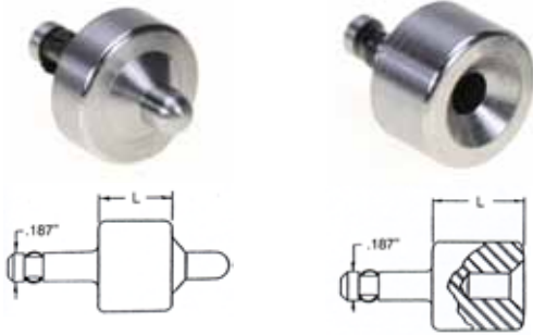
426XP Punch (Male)
