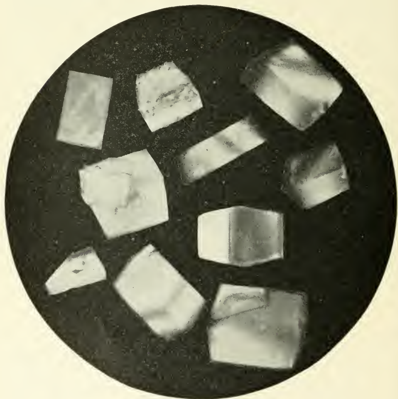
FIG. 343. Strychnine sulphate: tetragonal crystals in polarized light, showing side aspect.
