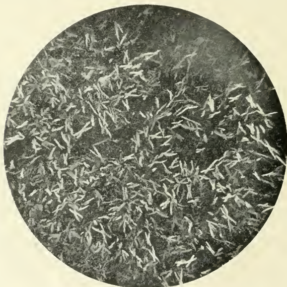
FIG. 332. Codeine: x-shaped skeleton crystals from 10 per cent. alcoholic solution.
