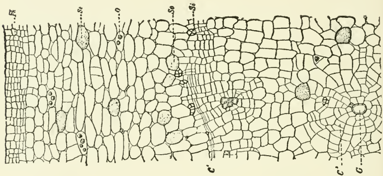
FIG. 195. Transverse section of jalap: Ph, cork cells; Se, resin cells; O, rosette aggregates of calcium oxalate; Si, sieve cells; G, tracheæ; C 1 , primary cambium; C 2 , secondary cambium.—After Meyer.
