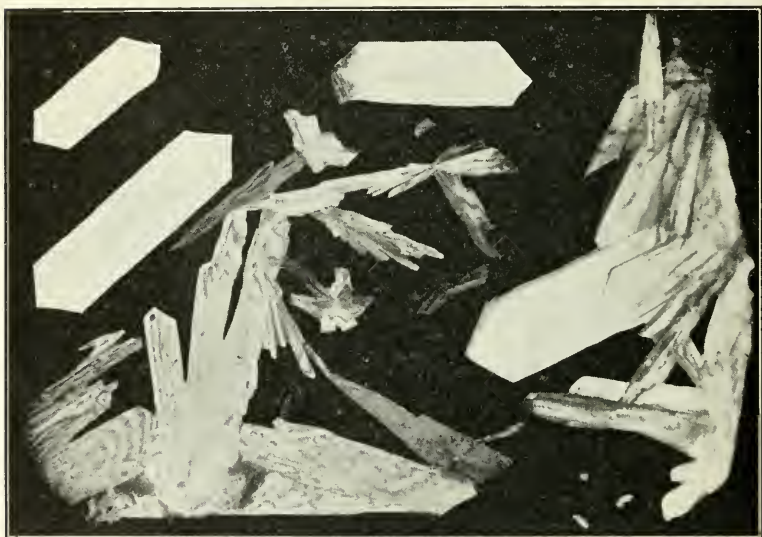
FIG. 331. Brucine sulphate: orthorhombic crystals from aqueous solution.
