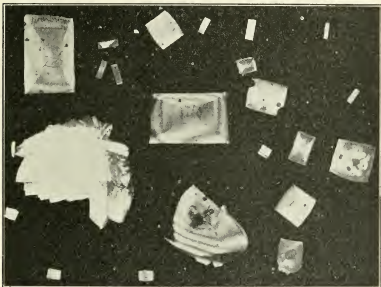
FIG. 154. Hematoxylin: monoclinic tabular crystals from aqueous solution.
