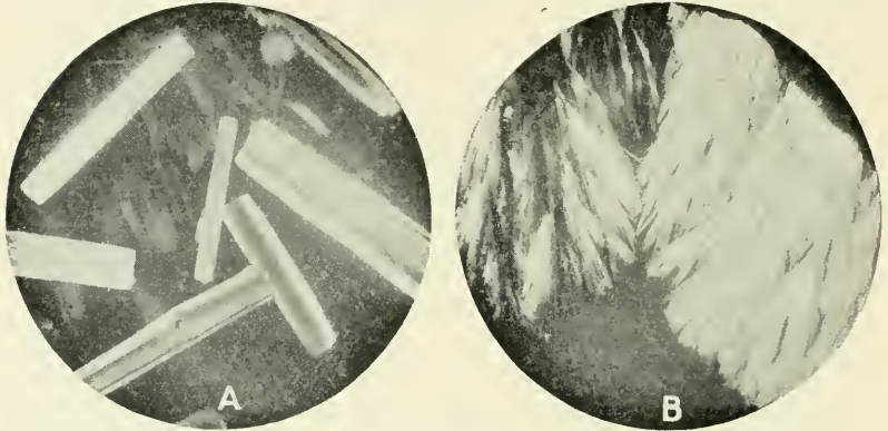
FIG. 149. Orthorhombic crystals of Mannitol (Mannit) obtained from aqueous solutions: A, large crystals; B, feathery aggregates of needles.
