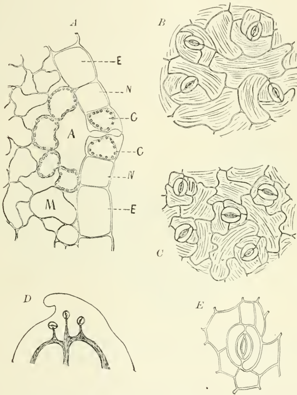
FIG. 106. Stomata and water-pores. A.—Transverse section through lower surface of leaf of stramonium; stoma, with guard cells (G), containing cytoplasm, nucleus and chloroplasts; N, surrounding cells; A, intercellular cavity usually filled with cell-sap or watery vapor; E, epidermal cells; M, mesophyll. B.—Surface section of upper surface of leaf of Viola tricolor showing four stomata. C.—Surface section of under surface of leaf of Viola tricolor showing five stomata. D.—A section through the margin of the leaf of Viola tricolor showing a tooth with three water-pores. E.—A water-pore of Viola tricolor in surface section.
