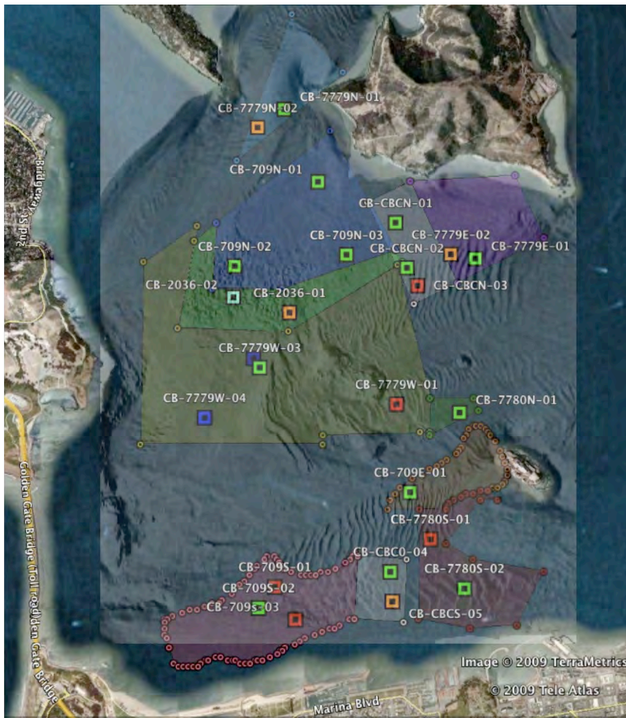
Figure 3-4. Overlay of survey station locations (squares) relative to standing sand waves and other seafloor microhabitats in Central Bay. Colors of square site symbols correspond to clusters in Figure 3-1.
