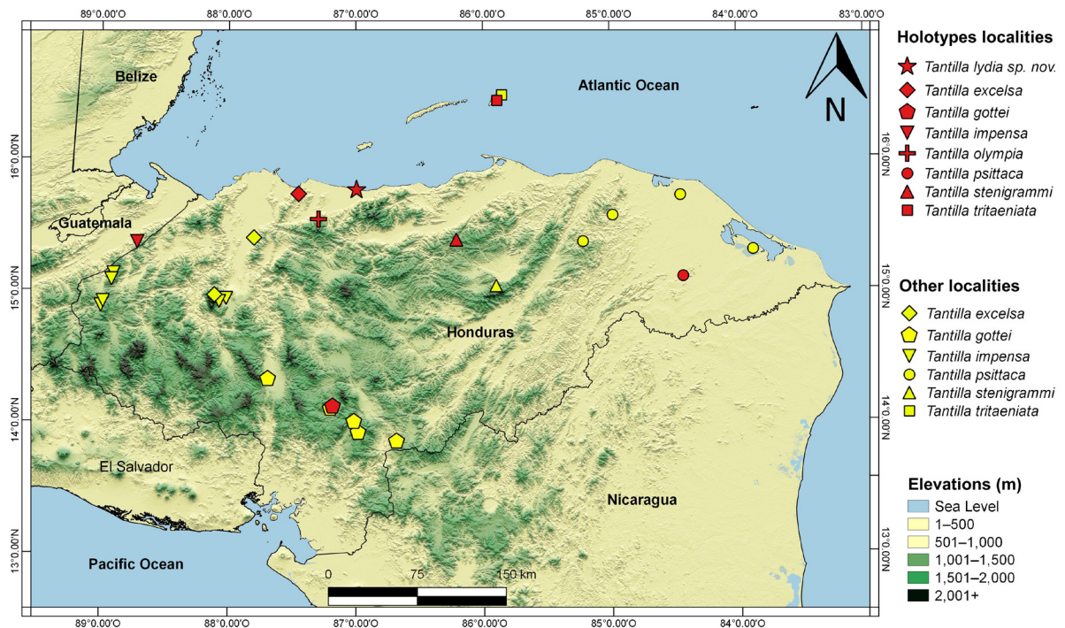
Fig. 3. Distribution of the species of the Tantilla taeniata group in Honduras. The star indicates the type locality of Tantilla lydia sp. nov. The most northwestern location of Tantilla gottei was recently published by Orellana Murillo et al. (2020).
