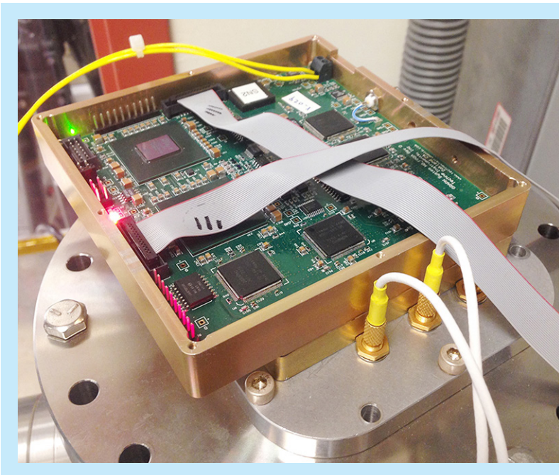
Fig. 10. Amplifier (bottom) and digitizer (top) boxes mounted to 50-mm detector backplate.
