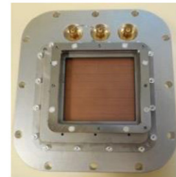
Existing 50-mm detector (without MCPs)
