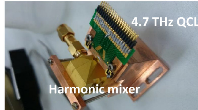
Array of DFB lasers at \sim 4.7\text{ THz} . The harmonic mixer is used to phase-lock the QCL LO.
