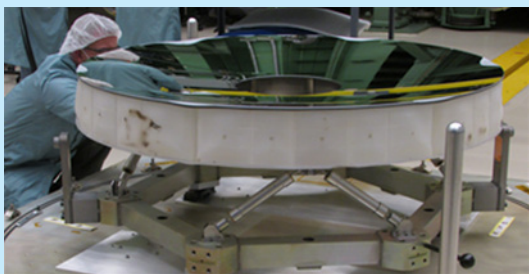
Fig. 3. Coated 1.5-m ULE® AMTD-2 mirror.
