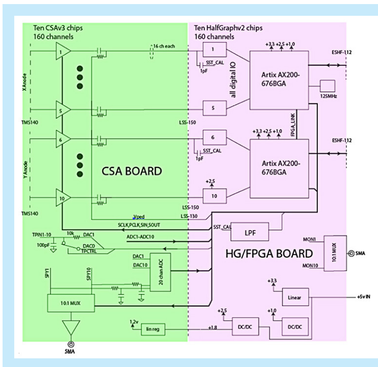
Fig. 9. High-level schematic of 50-mm detector electronics, including a 160-channel amplifier board (left) and 160-channel digitizer board with two FPGAs to control ASICs and calculate event centroids (right).
