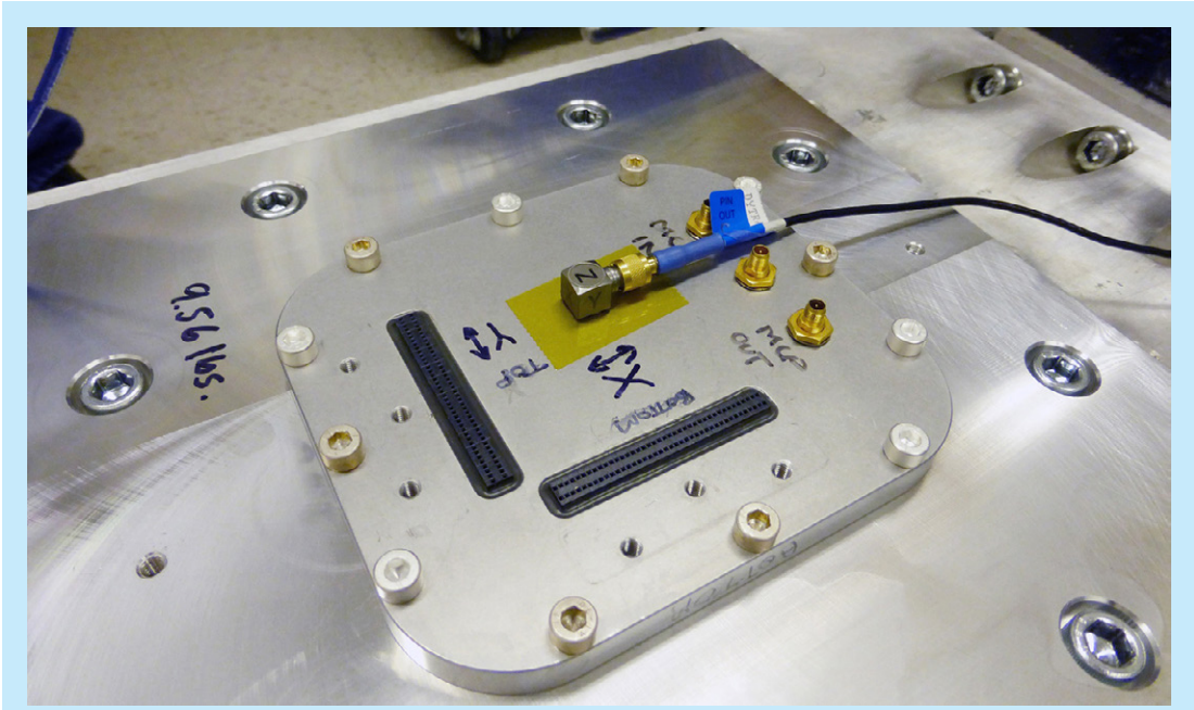
Fig. 19. 50-mm XS detector mounted on vibration table at SSL.
