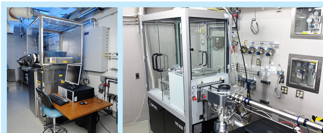
Fig. 6. ALD systems at JPL. Left: Oxford OpAl showerhead-style ALD reactor with gas feedthroughs and process controls enabling \text{AlF}_3 and \text{MgF}_2 coatings development. Right: Beneq ALD deposition system.
