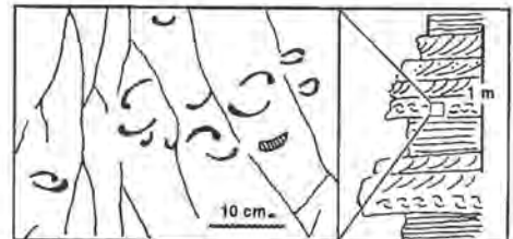
Text-FIG. 3. Simplified portion of a stratigraphic column of the Cáqueza Group, lower interval, measured in the railroad that leads to Tobia from Utica. This figure shows the coarse sandstones from where the fossils were collected, and a sketch of the arrangement of valves in the outcrop.
