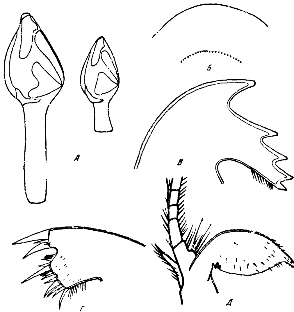
Fig. 1. Octolasmis warwickii , Nao Chau area.
