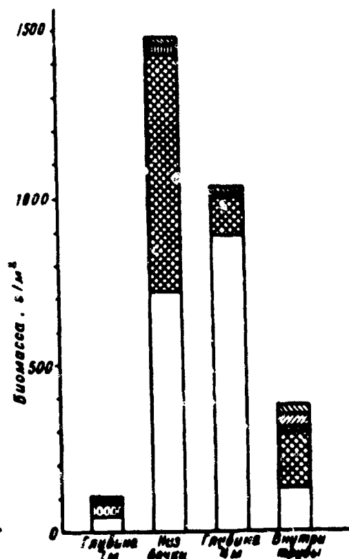
Fig. 7. The biomass of marine fouling on buoy Tsar'-banki.
