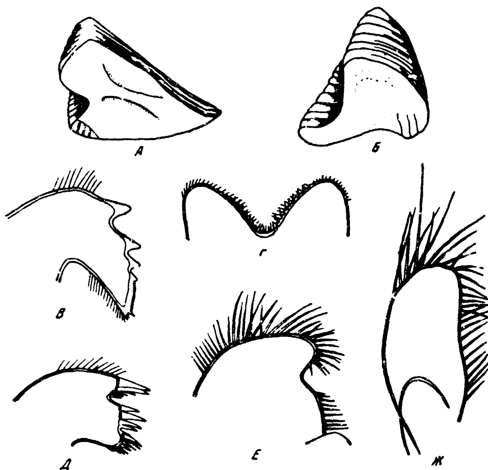
Fig. 2. Chthamalus challengeri , Lūta area.
