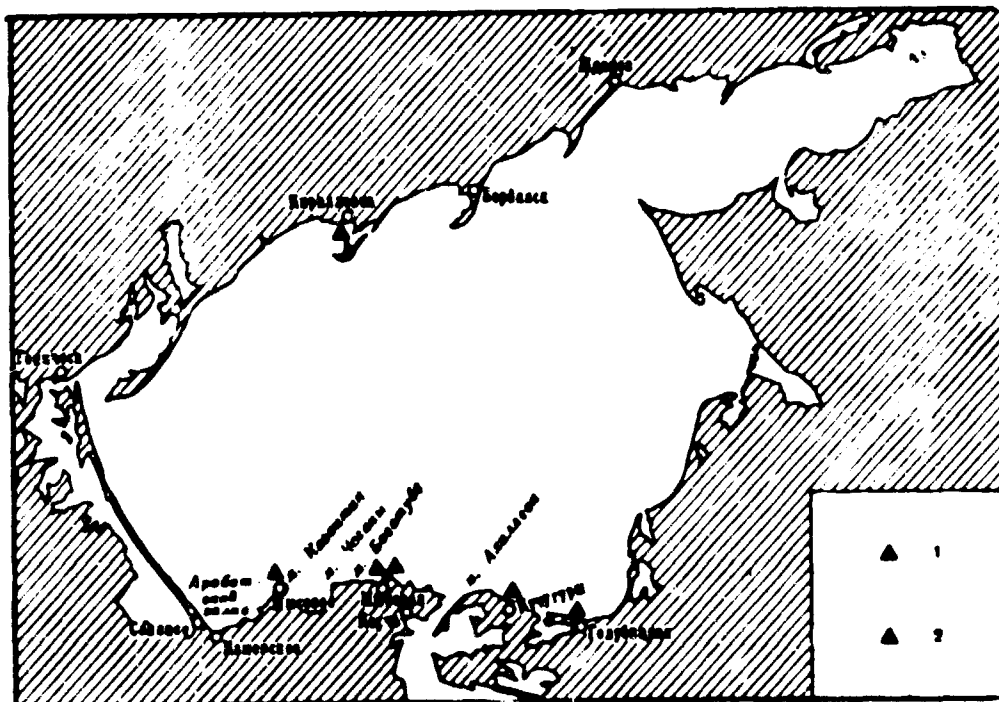
Fig. 2. The distribution of shipworms Tereedo navalis (1) and T. pedicellata (2) along the coast of the Sea of Azov.
