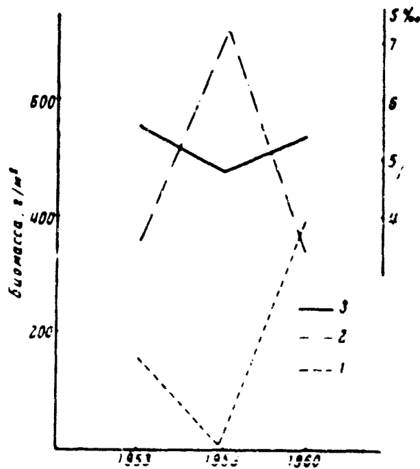
Fig. 3. The mean biomass of mytilaceans (1) and dreissenians (2) in the northern sector of the Caspian Sea, and the mean yearly salinity (3) in the surface layer in ostrova Tyuleniy area in 1953, 1958 and 1960.
