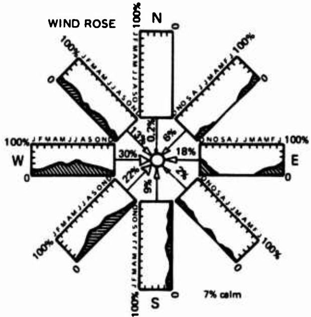
Figure 5. Climatological data for San Diego region. (Source: San Diego Unified Port District, 1972.)
