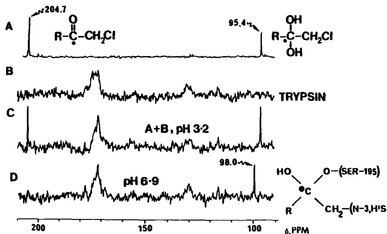
FIGURE 5. The ^{13}\text{C} -NMR spectra of (A) N^\alpha -carbobenzyloxylsilylchloromethylketone ( \text{RCOCH}_2\text{Cl} ); \bullet - ^{13}\text{C} , 90% enrichment; 47.6 mM (by weight); 1 mM HCl; \text{D}_2\text{O} , 16.7% (by volume); volume, 0.6 ml; 1660 accumulations; pH 3.1. (B-D) 20 mM sodium phosphate; 12.5 percent (by volume) \text{D}_2\text{O} ; 10,000 accumulations; trypsin, 0.28 mM (concentration of fully active enzyme); volume, 8 ml. The \text{RCOCH}_2\text{Cl} concentrations, pH and enzyme activities were as follows: (B) 0.00 mM, 3.2, 100%; (C) 0.38 mM, 3.2, 100%; (D) 0.37 mM, 6.9, 0.06%. All spectra were accumulated on a Bruker WM300 WB spectrometer at 75.4 MHz for ^{13}\text{C} nuclei.
