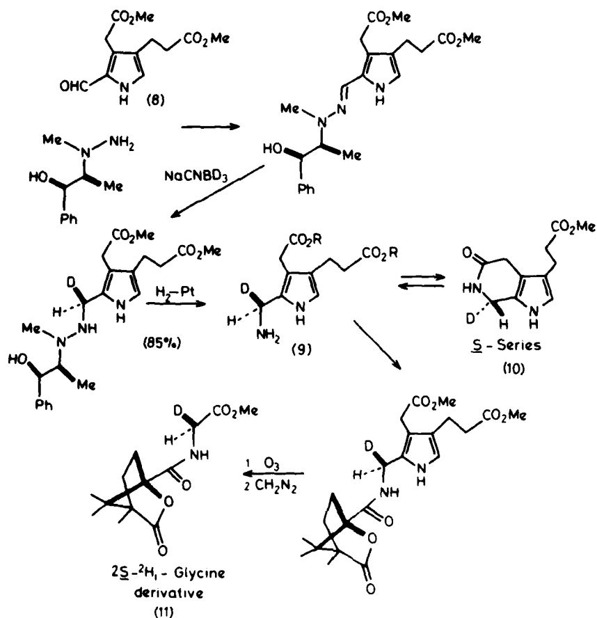
SCHEME 6
