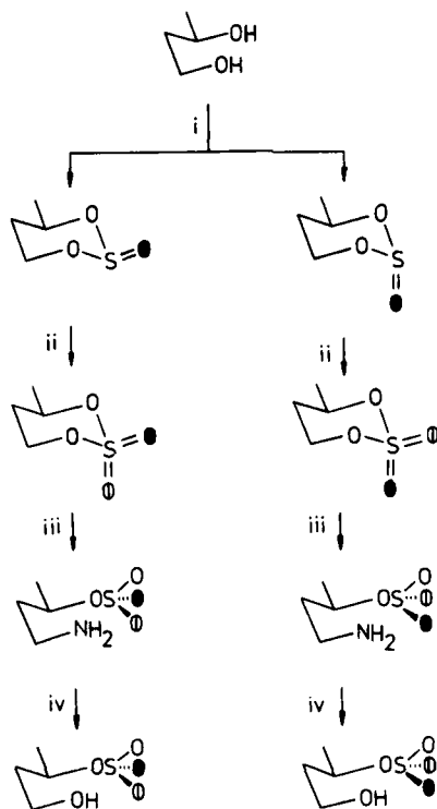
SCHEME 1. The synthesis of ( S )- and ( R )-3( R )-butan-1-ol-3-[ 16 O, 17 O, 18 O]sulfate. O = 17 O; ● = 18 O. Reagents: (i) S 18 OCl 2 , C 3 H 7 N; (ii) Ru 17 O 4 ; (iii) NH 3 , MeOH; (iv) NaNO 2 , aq. AcOH.
