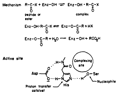
SCHEME 3. Serine transacylases.
