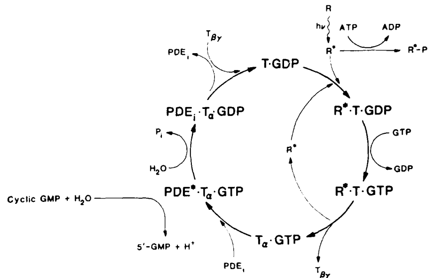
FIGURE 2. The cycle of reactions in rod outer segments initiated by bleached rhodopsin ( R^* ).
