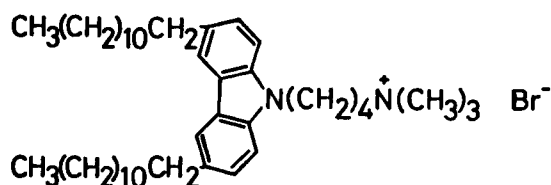
SCHEME 9. 2C 12 -Cz-C 4 N + .
