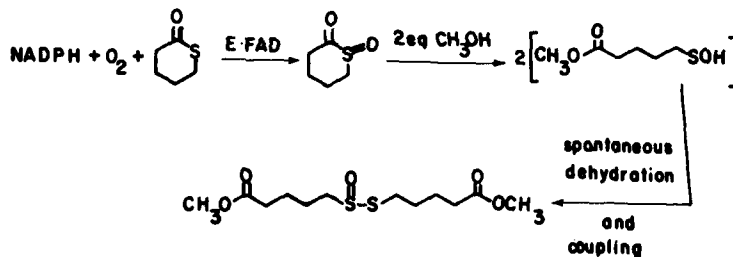
SCHEME 7
