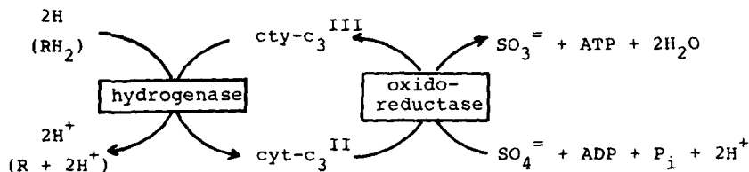
SCHEME 8. Simplified total chemical function of sulfate-reducing bacteria.
