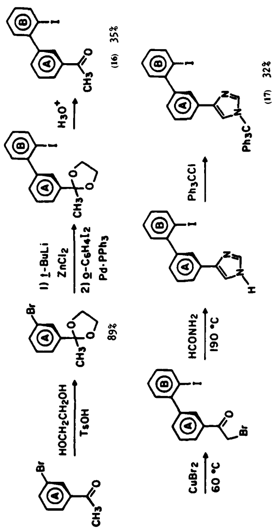
SCHEME 9. Syntheses.
