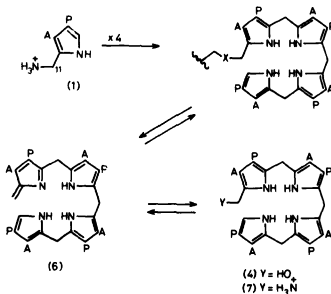
SCHEME 5
