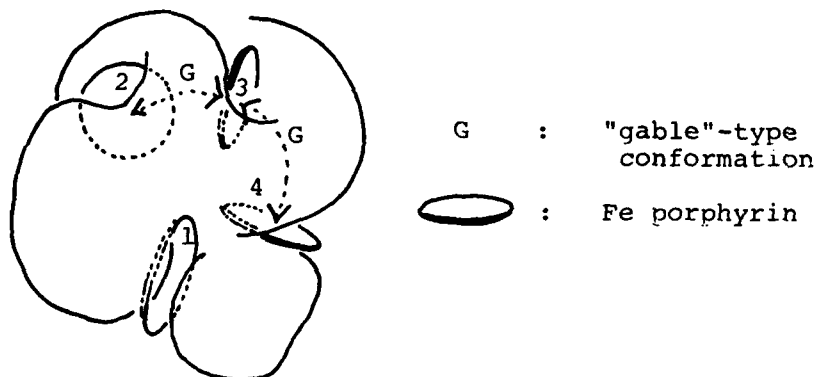
FIGURE 5. Conformational characteristics of four heme units in Cyt c_1 .
