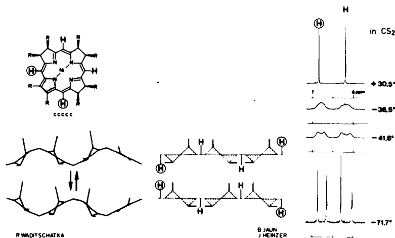
FIGURE 18. Conformational inversion barrier in ccccc-nickel(II)-octaethyl-pyrrocorphinato.
