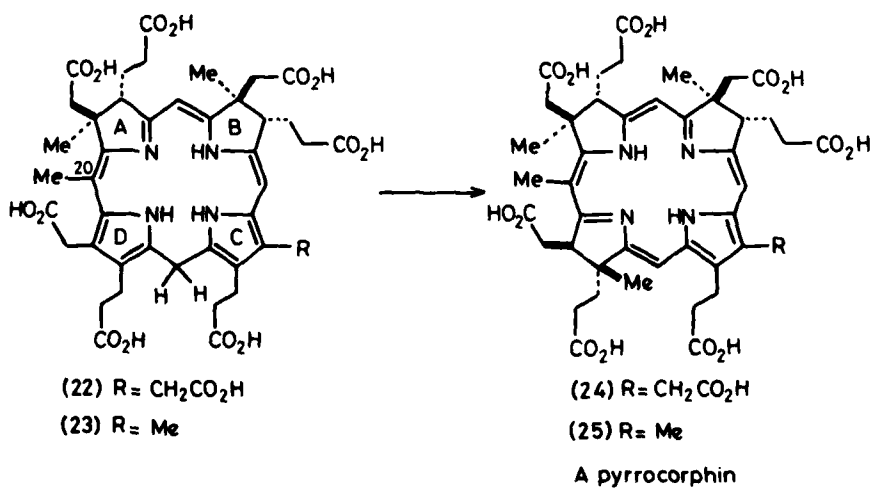
SCHEME 11
