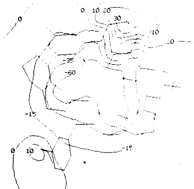
FIGURE 1. The electrostatic potential pattern of the cyclic urea mimetic of \alpha -chymotrypsin calculated in the z = -2 \text{ \AA} plane. The molecule is oriented so that its anisole oxygens are in the z = 0 plane. The coordinates are taken from the enzyme mimetic-substrate complex calculated by molecular mechanics. In this orientation, the oxygen atom of the m -methylenedioxy substituent is found at z = -3.7 \text{ \AA} (in the lower left-hand corner of the figure) and the coordinates of the substrate are between z = -1.2 and -5.5 \text{ \AA} . The electrostatic potential is calculated as the Coulombic interaction between a positive point charge in the plane and the static charge distribution of the molecule modeled by atomic point charges positioned at the nuclei, as described in ref. 1. Equi-energy contours are given in units of kcal/mole.
