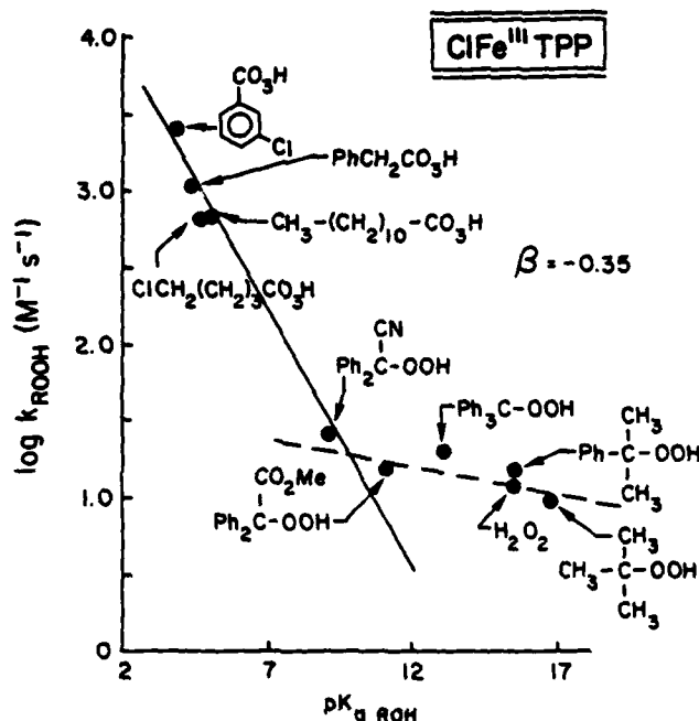
FIGURE 2. Plot of \log k_{\text{ROOH}} vs. pK_a of corresponding ROH. The reactions were studied under an argon atmosphere in spectral grade methanol employing collidine buffer at pH 6.5 (collidine/collidine \cdot HCl = 0.126); k_{\text{ROOH}} was determined from the intercept of plots of k_{\text{obs}} vs. collidine at zero collidine buffer concentration. Values of k_{\text{ROOH}} so determined are in close agreement with rate constants determined in methanol without buffer present. \text{ClFe}^{\text{III}}\text{TPP} = (0.15-1.5) \times 10^{-4} M; [\text{TBPH}] = 0.1-0.3 M; [\text{ROOH}] = (0.2-1.5) \times 10^{-2} M; T = 30^\circ\text{C} .
