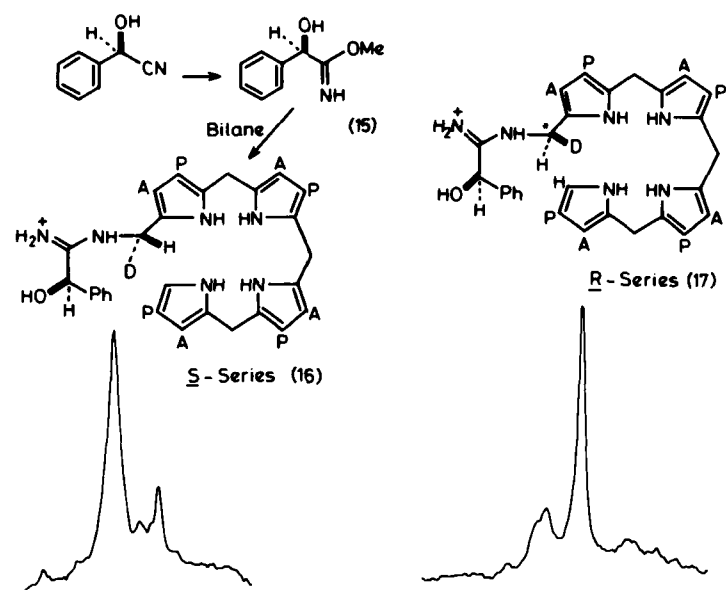
SCHEME 8
