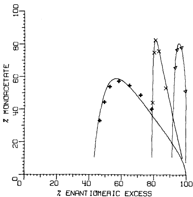
FIGURE 2. Plot of percent monoacetate vs. percent enantiomeric excess (ee). PLE with: 18, +—+; 26, x—x; 32, Δ—Δ. The curves are computer generated using the values of \alpha , E_1 , and E_2 given in the text; +, x, and \Delta are experimentally determined values.
