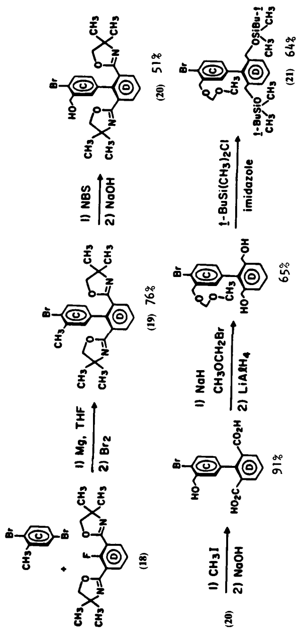
SCHEME 10. Syntheses.
