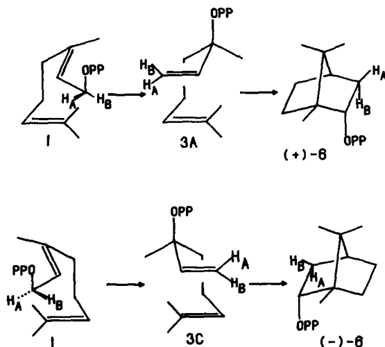
SCHEME 7. Enzymatic conversion of 1 S -[1- 3 H]geranyl pyrophosphate ( H_A = T, H_B = H ) and 1 R -[1- 3 H]geranyl pyrophosphate ( H_A = H, H_B = T ) to (+)- and (-)-bornyl pyrophosphate (6) with net retention of configuration.
