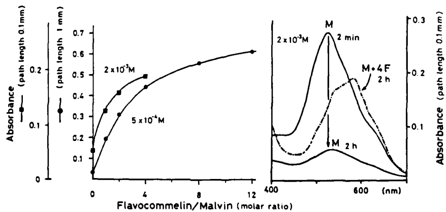
FIGURE 6. Effect of flavocommelin concentration on absorbance at \lambda_{max} of malvin at pH 6.0, 2 hours after dissolving. Concentrations: 5 \times 10^{-4} \text{ M} (●); 2 \times 10^{-3} \text{ M} (■).
