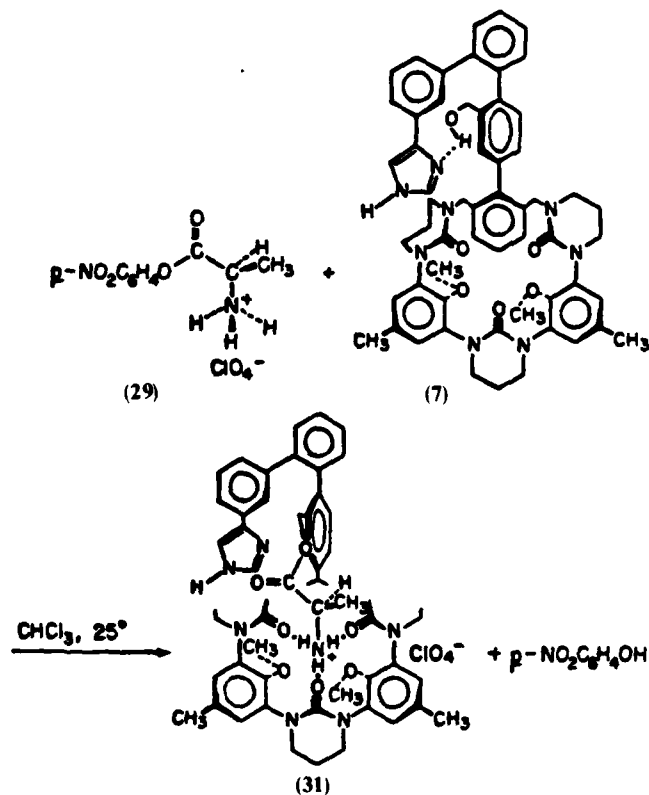
SCHEME 16. Templated transacylation.
