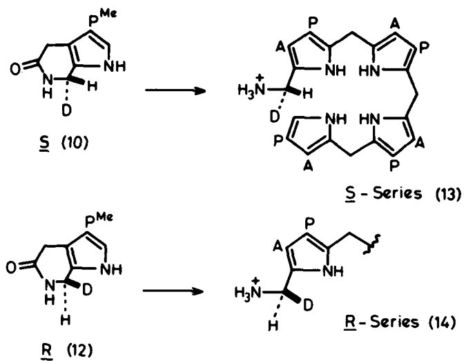
SCHEME 7
