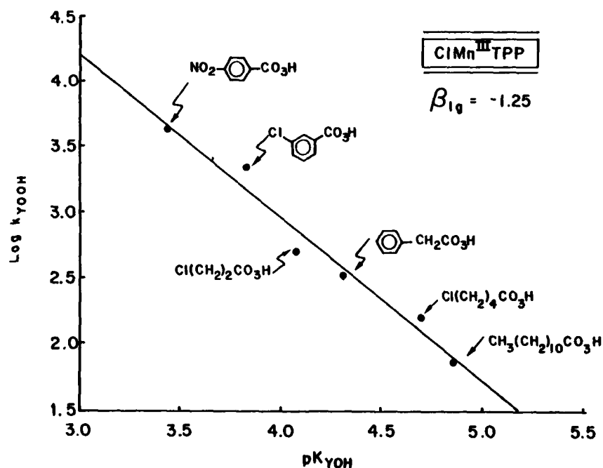
FIGURE 3. Plot of the second-order rate constants ( k_{YOOH} ) for the reaction of \text{ClMn}^{\text{III}}\text{TPP} with percarboxylic acids (YOOH) vs. pK_a of the carboxylic acid leaving groups ( pK_{YOH} ).
