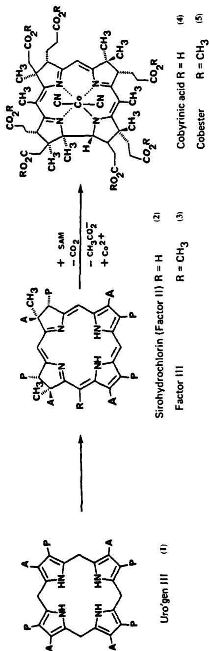
SCHEME 1
