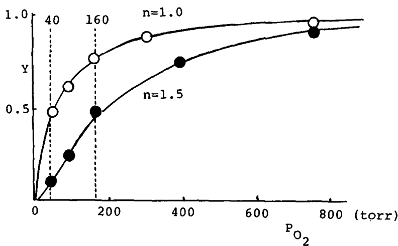
FIGURE 10. Partial O_2 pressure vs. fractional saturation. ○: (TPP) - Co^{II} (L); ●: (gable) Co_2^{II} ( \frac{1}{2} ); -20^\circ C , DMN. [Co^{II} (gable)] = 2.0 \times 10^{-6} M, [L-L] = 15 \times 10^{-3} M; Co(TPP) = 2.0 \times 10^{-6} M, [L] = 0.04 M.
