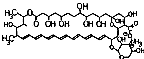
SCHEME 4. Amphotericin B.
