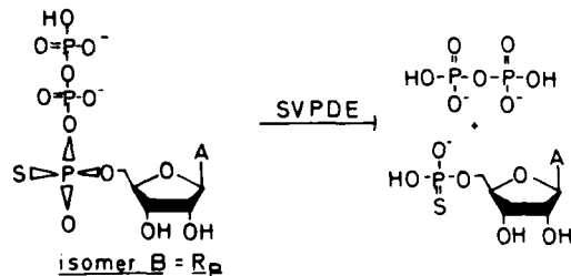
FIGURE 2. Determination of absolute configuration of ATP α S. (From Eckstein et al. 37 Reprinted by permission from Methods in Enzymology. )
