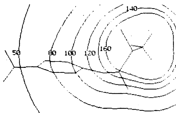
FIGURE 2. The electrostatic potential of the L-alanyl p -nitrophenyl ester cation substrate of the artificial enzyme in FIGURE 1. The electrostatic potential is calculated in the z = -2 \text{ \AA} plane. The coordinates are taken from the enzyme mimetic-substrate complex, oriented as described in FIGURE 1. In this orientation, the nitrogen of the ammonium group is found at z = -2 \text{ \AA} , the carbonyl carbon is at z = -3.3 \text{ \AA} , and the nitrogen of the nitro group is at z = -4.5 \text{ \AA} . Equi-energy contours are given in units of kcal/mole.
