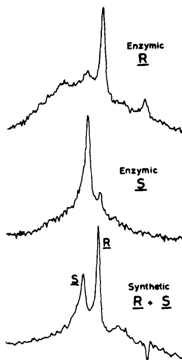
FIGURE 2. ^1\text{H-NMR} signals (400 MHz) from derivatized aminomethylbilanes from enzymic experiments using R -PBG (upper signals) and S -PBG (center signals). The lower signals are from a mixture of the synthetic derivatized S and R bilanes (16) and (17), containing more of the latter.
