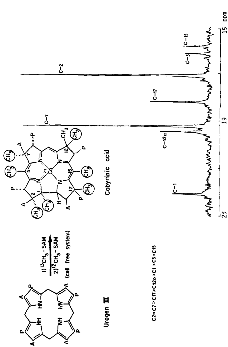
FIGURE 1. Broad band, 125 MHz, ^1\text{H} -decoupled (1 w), ^{13}\text{C} -NMR spectrum of ^{13}\text{C} -enriched cobester (5), 270 \mu\text{g} in 0.5 ml KCN saturated benzene- d_6 , isolated from P. shermanii (see text for incubation details). Chemical shifts are with respect to tetramethylsilane (TMS) at 0 ppm. Spectral parameters: spectral width, 30 ppm; pulse repetition rate, 0.7 s; \alpha = 65^\circ . Spectrum represents the sum of 51,382 free-induction decays (FIDs) with 2.0 Hz line broadening.
