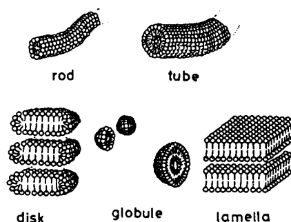
FIGURE 1. Schematic illustrations of the representative morphologies of bilayer aggregates.
