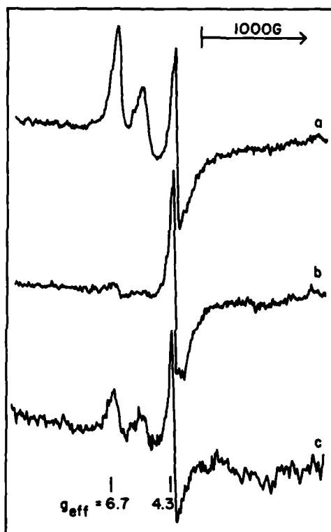
FIGURE 1. Reduction of PAH with 6MPH 4 . (a) Paramagnetic resonance spectrum of PAH (78 μM, specific activity = 6.5, 0.8 iron per subunit, pH 7.2, 4°C) at 5 K. Instrument settings as follows: modulation amplitude 20 gauss; receiver gain 2 \times 10^4 ; microwave power 0.1 mW; time constant 0.25 s; scan time 8 min; scan range 0.4 to 2.4 kgauss. Values of prominent spectral features are given. (b) EPR spectrum at 5 K of PAH (62 μM, specific activity = 2.4) after the addition of half an equivalent of 6MPH 4 . Instrument settings are the same as in (a). (c) EPR spectrum of the sample described in (b) after treatment with Sephadex to remove 7,8-dihydropterin (54 μM PAH, specific activity = 2.5); instrument settings were as described for (a), except time constant 0.5 s, scan time 16 min, gain 4 \times 10^4 .
