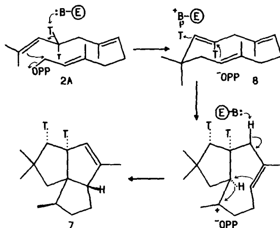
SCHEME 8. Conversion of [9- 3 H 2 ,12,13- 14 C]farnesyl pyrophosphate, folded in conformer (2A), to pentalene (7), via humulene (8) with retention of the proton derived from C-9 of farnesyl pyrophosphate.
