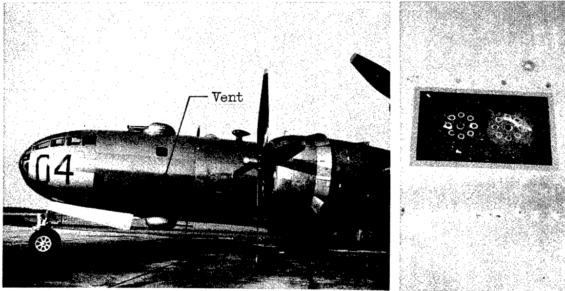
Figure 9.- Fuselage static-pressure vents on airplane I.
