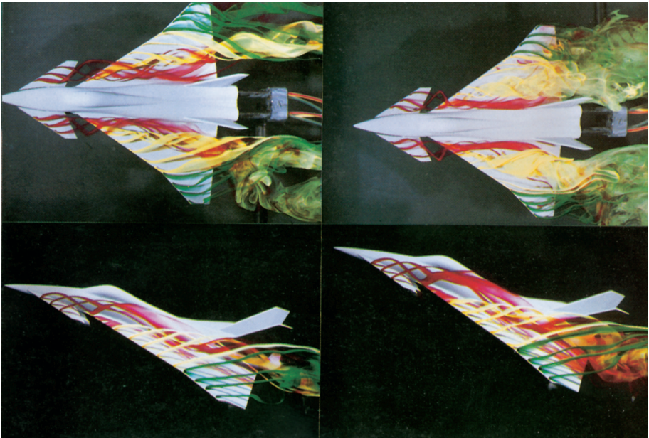
Water tunnel flow visualization illustrates the vortex flow structure over the wing of a highly swept canard-wing-body fighter configuration at two angles of attack. (From MBB)
