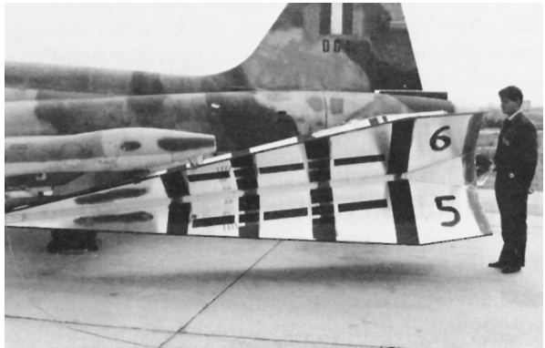
The Flight Mechanics Panel sponsored a project to help Greece develop a capability in store separation techniques. Although intended mainly for bombs and pods, it was also used for a Dart towed target, as shown here.
