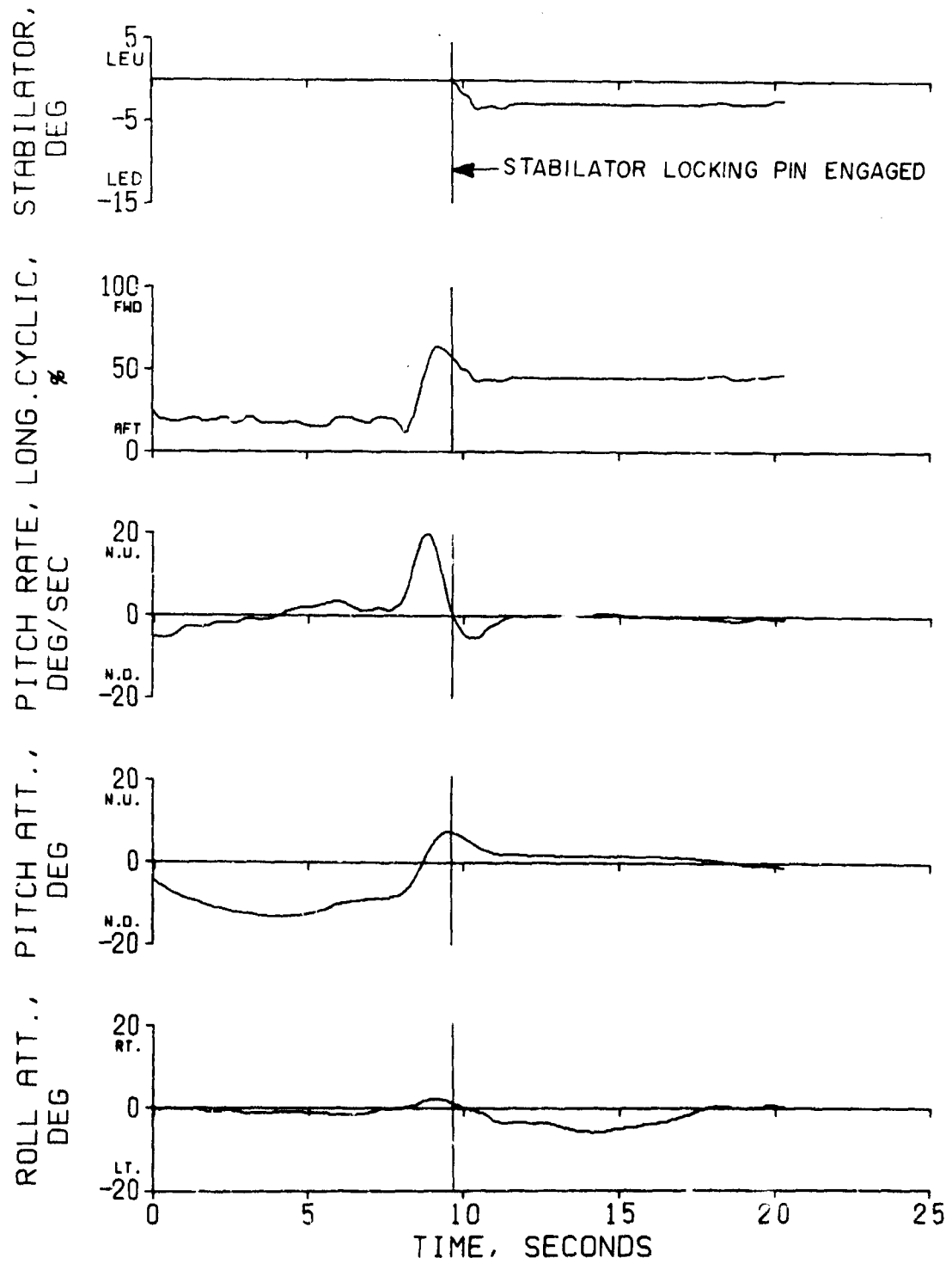
Figure 9. Time History of Aircraft and Control Motions During a Takeoff Transition Flight With Stabilator Coupled to "Fly" Mode at 40 Kn; Bias = -2.5 Deg, G.W. = 17,300 lb. C.G. = 256 In.
