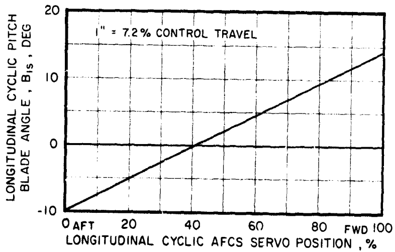
(a) LONGITUDINAL CONTROL RIGGING
