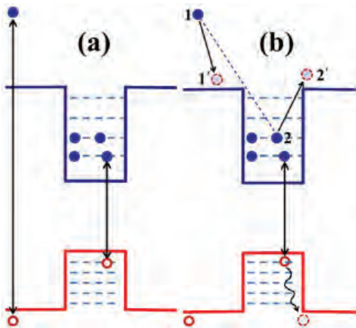
FIG. 5. Extraction of electrons localized in QD by hot electron that is excited by high-energy photon.
