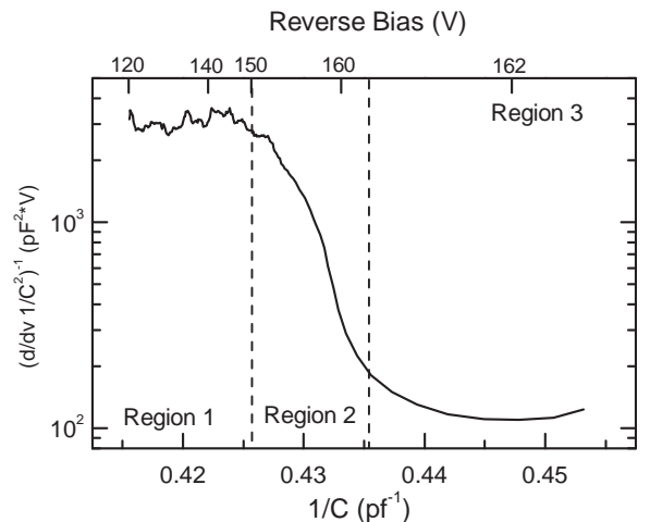
FIG. 2. CV characteristics for APD15.
