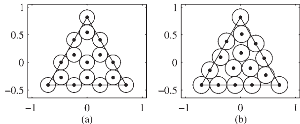
Fig. 2. Constellation designs for 16-CSK: (a) IEEE design and (b) optimized design.
