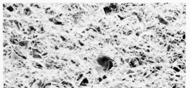
Ground with 177 μm SiC, no etching
