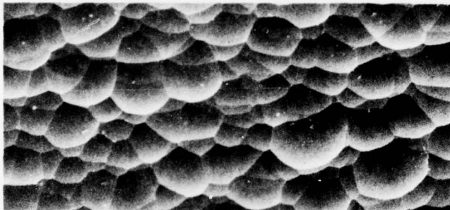
Ground with 22 μm Al 2 O 3 and 1.0-hour HF etch
