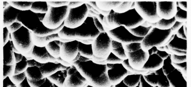
Ground with 177 μm SiC and 0.5-hour HF etch
