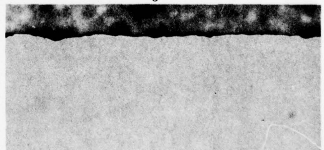
Ground with 9 μm Al 2 O 3 and 2.5-hour HF etch
