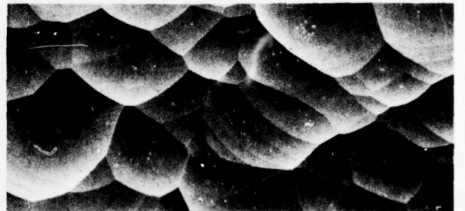
Ground with 177 μm SiC and 2.0 hour HF etch
