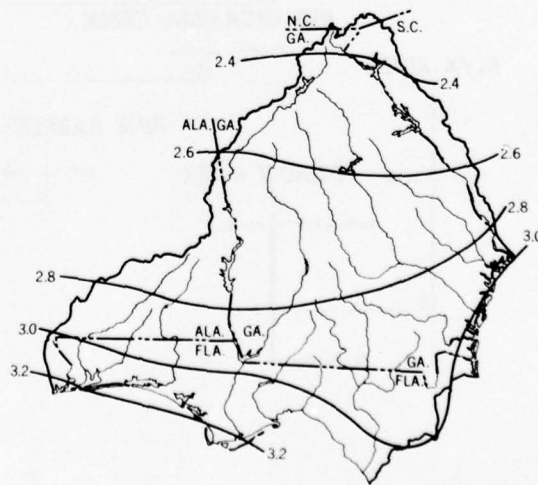
Figure 3.13 10-Year, 1-Hour Rainfall, Inches.
