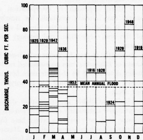
OCMULGEE RIVER AT MACON, GEORGIA 1910—1958
