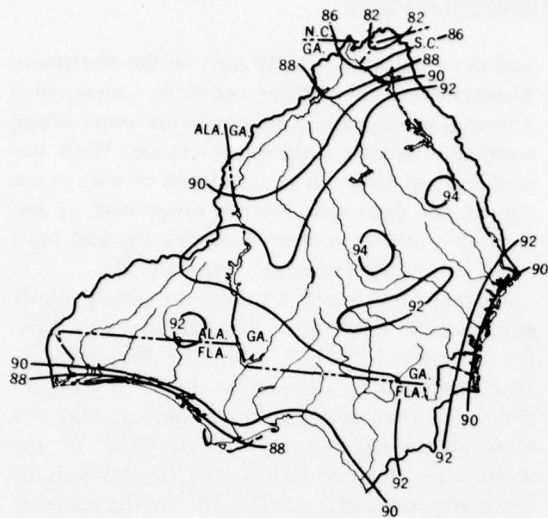
Figure 2.8 Average July Maximum Daily Temperature, °F.
