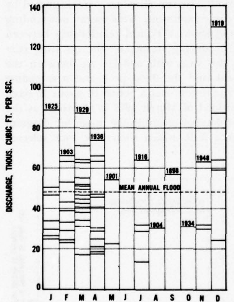
CHATTAHOOCHEE RIVER AT WESTPOINT, GEORGIA 1897—1958 REGULATED BY BUFORD RESERVOIR SINCE JAN., 1956
