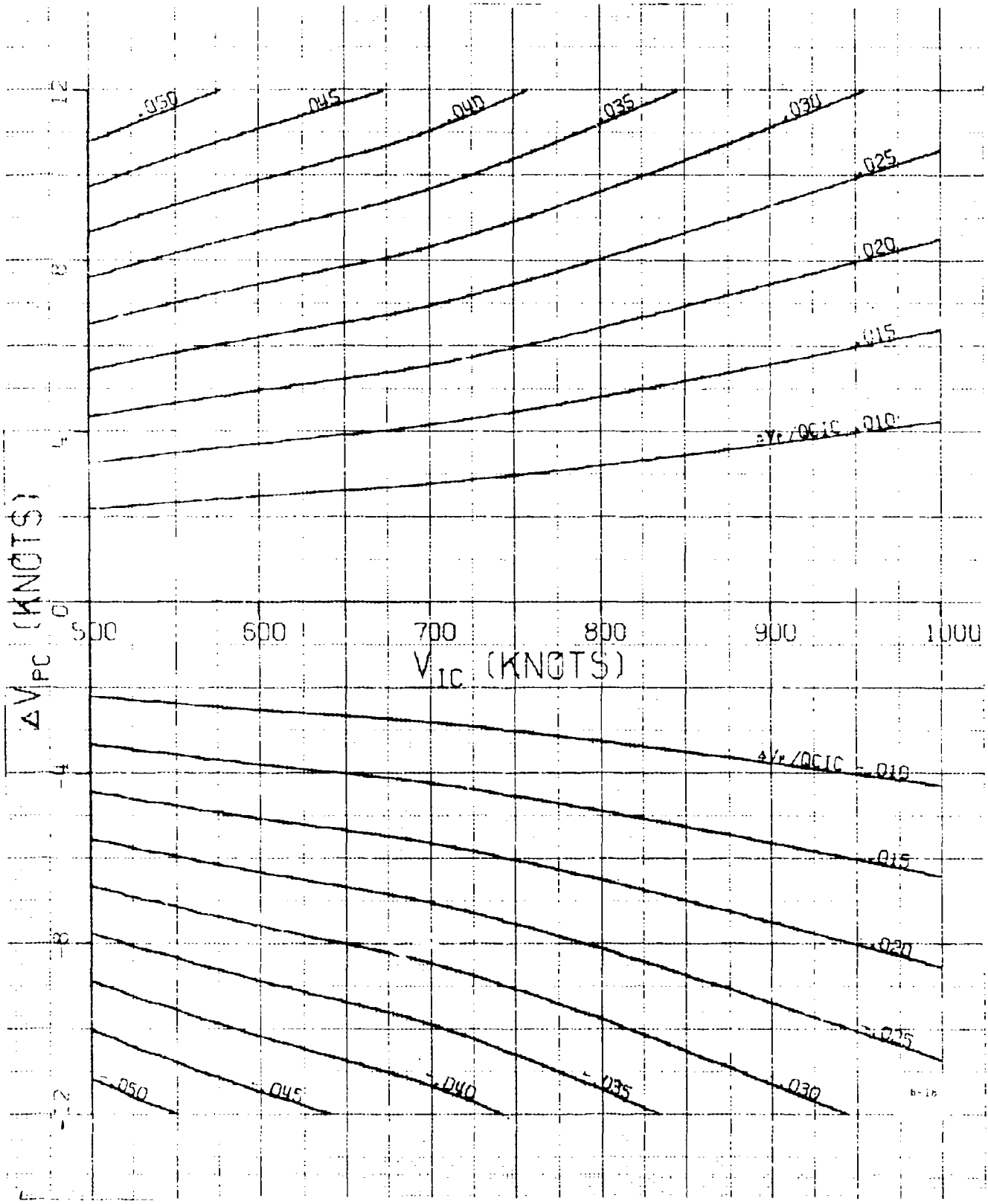
\Delta V_{PC} vs V_{IC} \frac{\Delta P_P}{\Delta C_{IC}} = \text{CONST}
