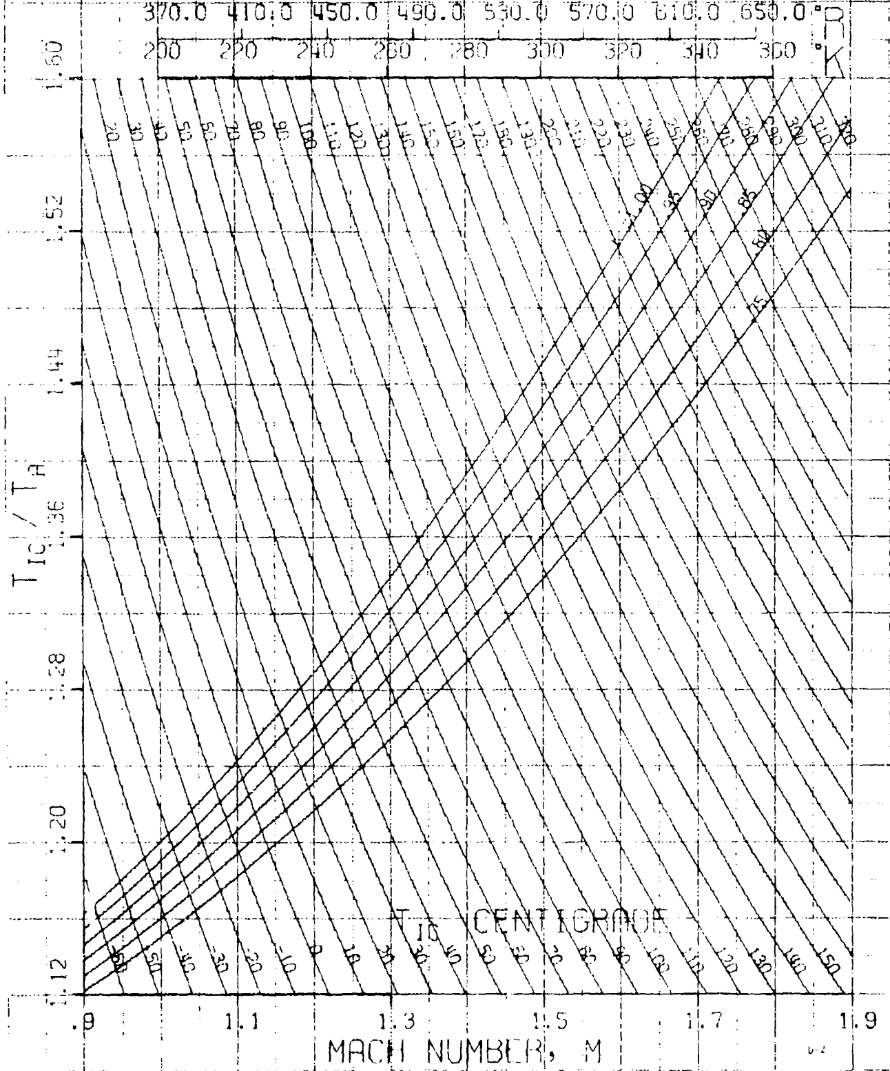
T_{IC} / T_A vs MACH
