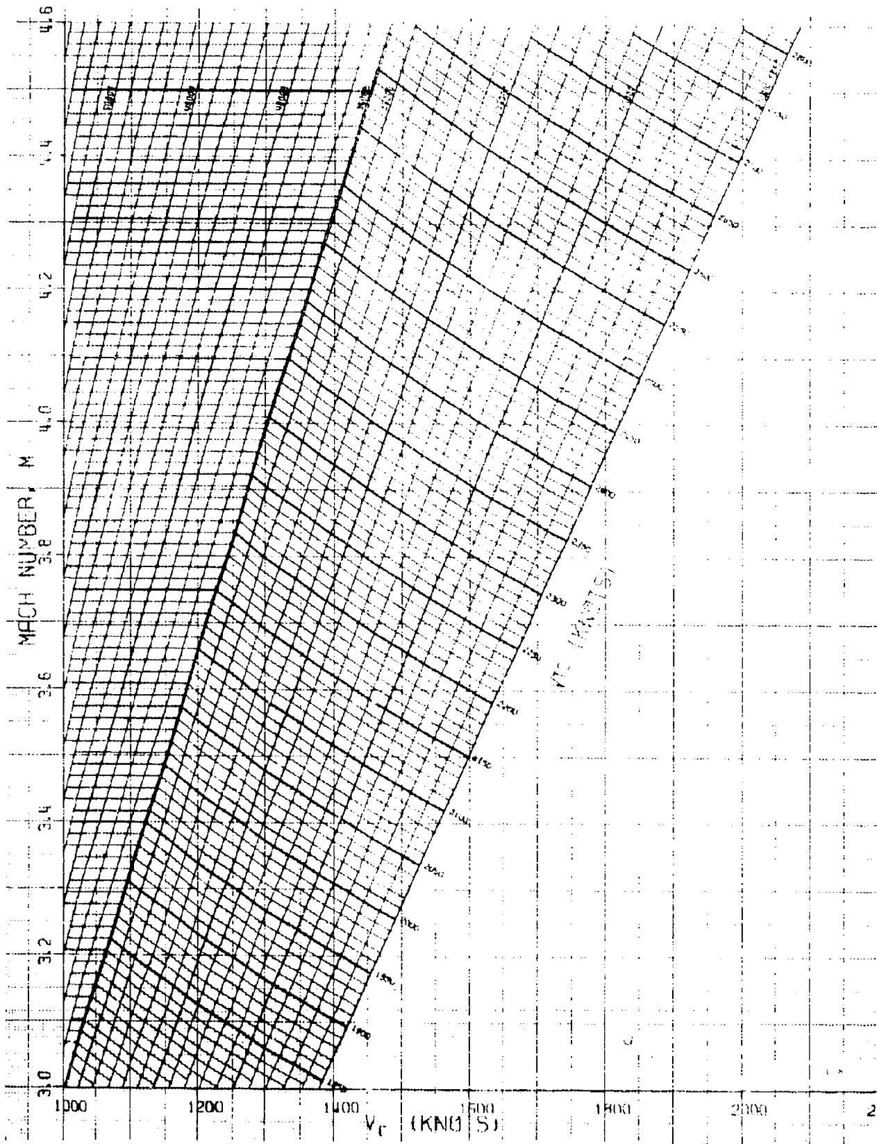
MACH vs V c
