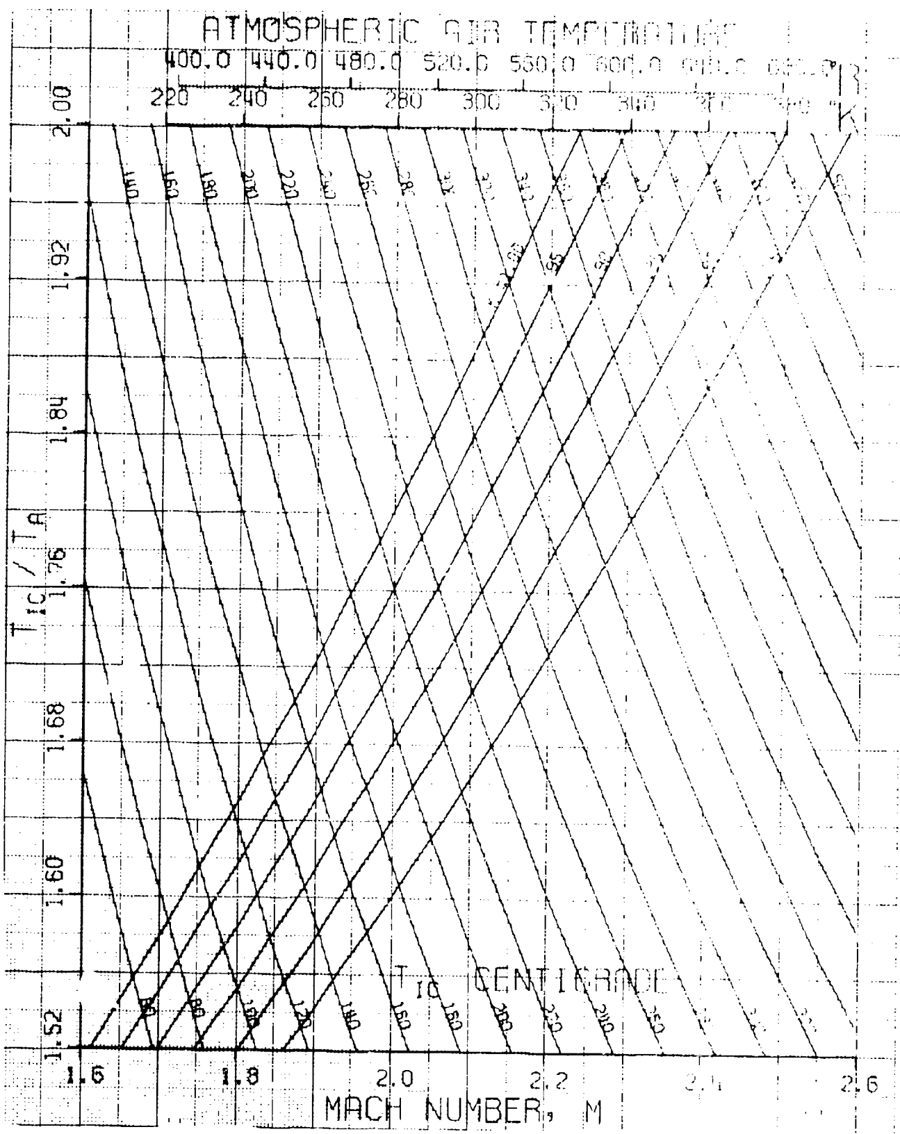
T_{IC}/T_A VS MACH
