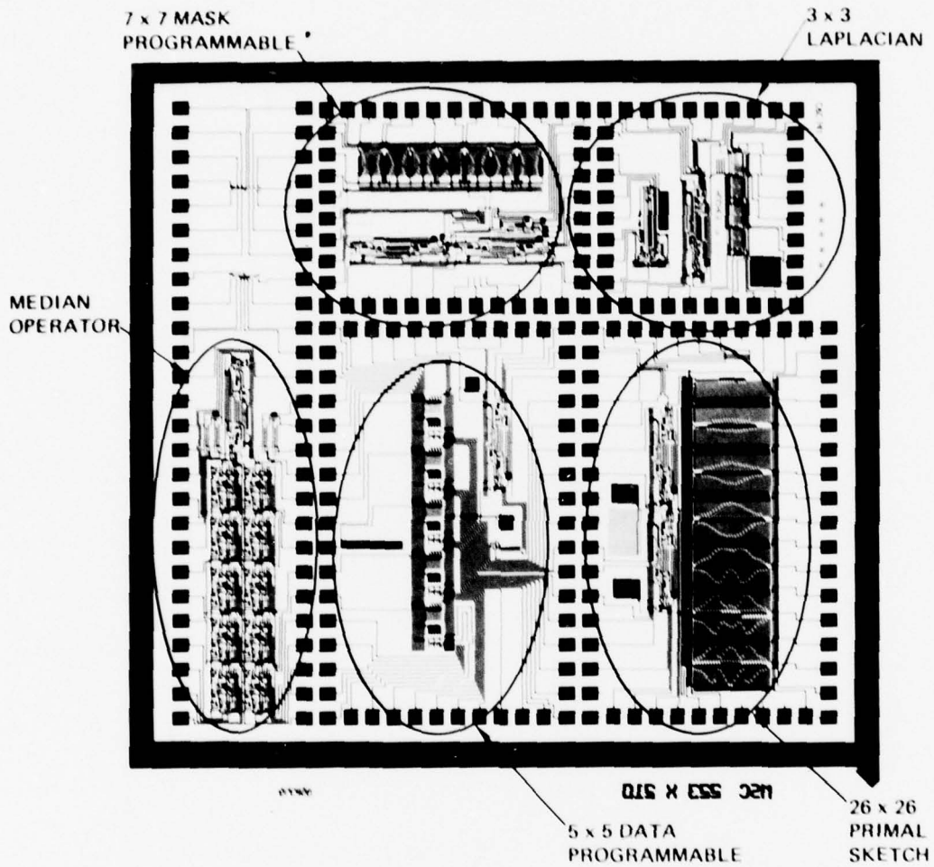
Figure 7. Photomicrograph of image understanding chip 111.
