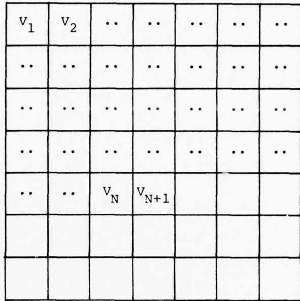
Two-dimensional Synthesis
