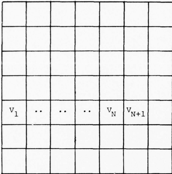
One-dimensional Synthesis
