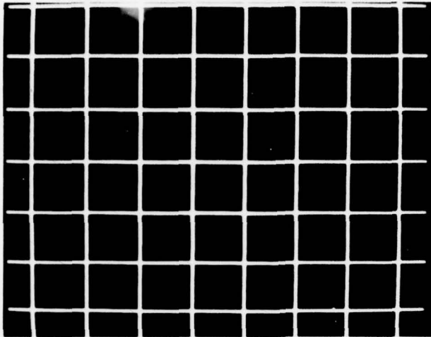
ORIGINAL
