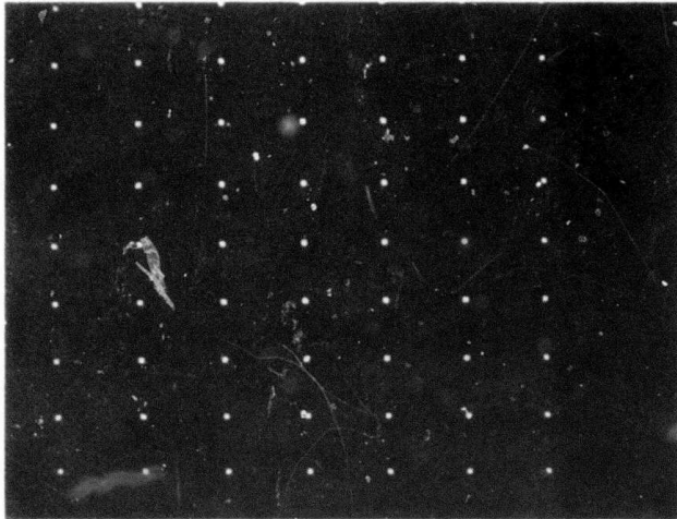
INPUT SIGNAL
