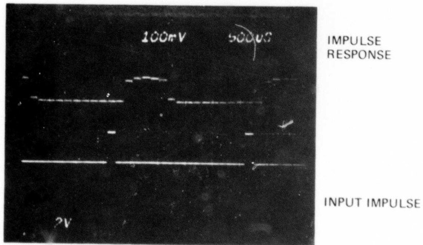
Figure 12. Impulse response of programmable array for setting (0, -1, 0, -1, 0) , (0, 1, 0, -1, 0) , and (1, 1, 1, 1, 1) .
