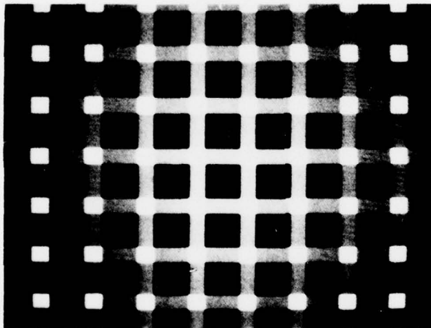
COMPUTER PROCESSED
