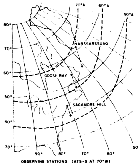
Fig. 1. The ionospheric (350-km altitude) intersections of the ray paths from ATS 3 located at 70°W to the observing sites at Sagamore Hill, Goose Bay, and Narssarsuaq.
