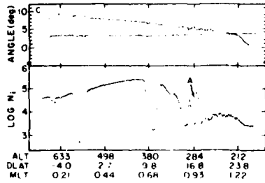
Fig. 1. Ion drift meter data from Al-C orbiter 2282. The observed pitch and yaw angles are shown in the upper and lower curves of the top panel, and the total density on the bottom. Positive angles correspond to ions moving up or left with respect to the spacecraft [after McClure et al., 1977].
