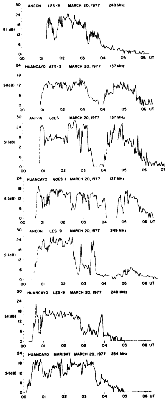
Fig. 6. Temporal variation of scintillation index S_1 in decibels, recorded at Ancon and Huancayo on March 19–20, 1977, by the use of transmissions from various geostationary satellites. The panels are arranged in order of decreasing west longitude of ionospheric intersection points of the various ray paths as shown in Figure 1.
