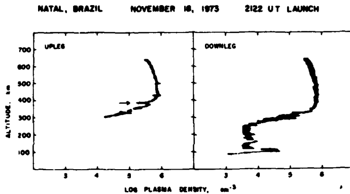
Fig. 2. Upleg and downleg plasma density profiles obtained on a sounding rocket during equatorial spread F. The arrow shows the locations of a deep depression in plasma density [after Kelley et al., 1976].
