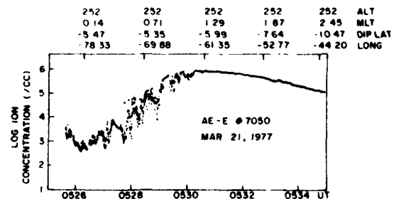
Fig. 13. Same as in Figure 10 for the AE-E orbit 7050 crossing the longitude interval of interest around local midnight.
