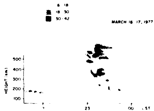
Fig. 5 Backscatter records of March 16-17, 1977. The irregularities maintain medium-level intensity from ~2300 to 2330 LST, at heights of 300-600 km, then disappear at the lower altitudes and trail off in intensity at the higher altitudes until 0030 LST
