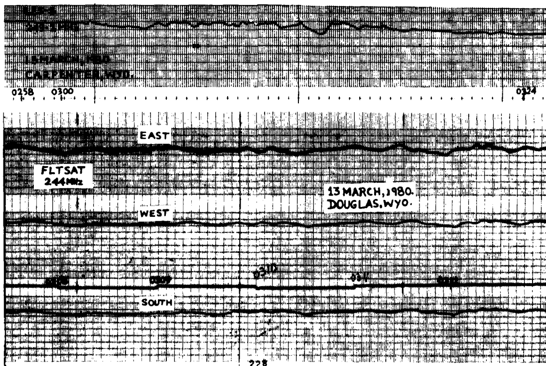
Figure 5. Same as in Figure 2 except for underdense heating on March 13, 1980. The AFS-3 data showed no effect and is not shown. The transmitter was in CW operation with power of 1.5 MW at 9.9 MHz between 0300-0315 UT. The critical frequencies at 0252 UT, 0310 UT and 0316 UT being 9.2, 8.5 and 8.35 MHz respectively
