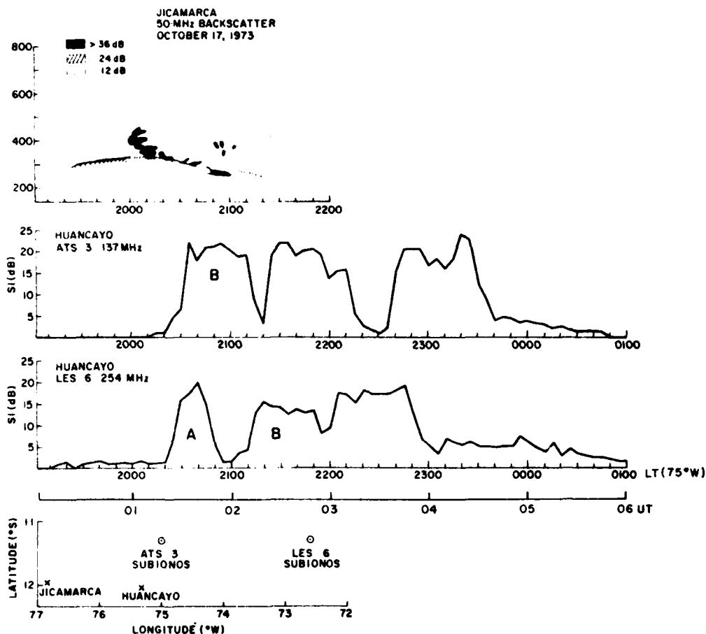
Fig. 4. Comparison of the 50-MHz radar backscatter map obtained at Jicamarca on October 17, 1973, and scintillation measurements made at Huancayo with the 137- and 254-MHz transmissions from the ATS 3 and Les 6 satellites, respectively.
