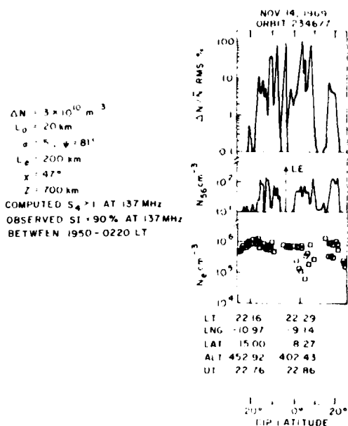
Fig. 3. Oyo 6 orbit showing equatorial electron density and rms amplitude of ionospheric irregularities in the Legon (Ghana, longitude sector) during a strong VHF scintillation event. The scintillation model parameters are also indicated [after Basu and Basu, 1976].
