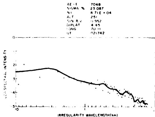
Fig. 9. Same as in Figure 7 for the sample shown in Figure 8.
