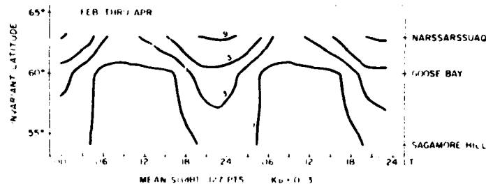
Fig. 8. Variation of mean seasonal scintillation index during the vernal equinox in decibels at 137 MHz with local time and invariant latitude derived from 127 values for each hourly data point at the three stations under quiet magnetic conditions ( Kp = 0-3 ).
