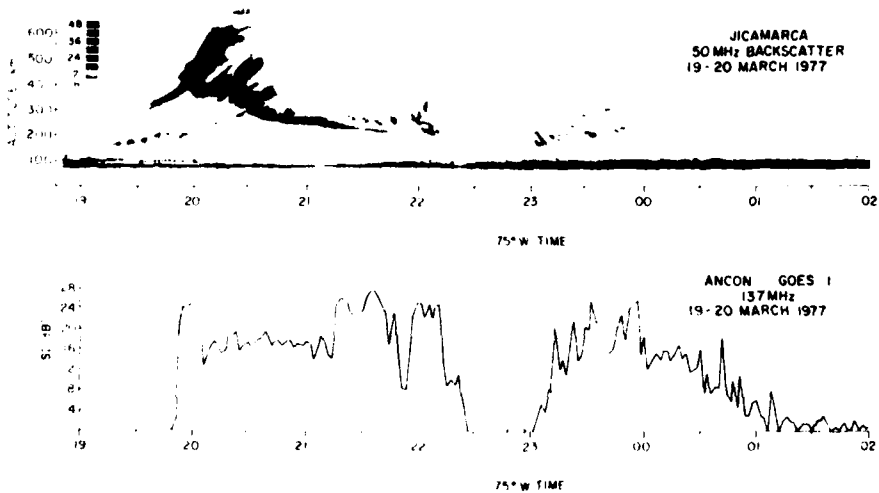
Fig. 6. Temporal variation of 50-MHz radar backscattered power obtained at Jicamarca and scintillation index, SI(dB), of 137-MHz transmissions from the Goes I satellite recorded at Ancon on March 19-20, 1977. Both sets of data refer to a nearly common ionospheric volume [after Basu et al. , 1978b].
