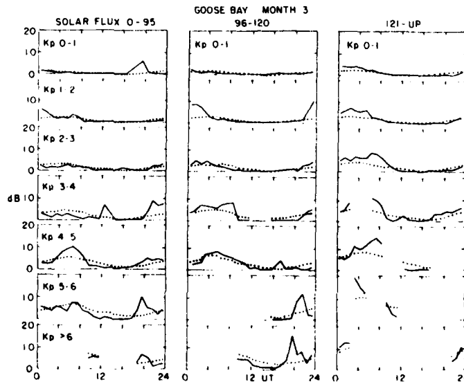
Fig. 3. Sample of behavior of data (solid curve) and the best-fitting model (dashed curve) in UT at Goose Bay as a function of different K_p and solar flux groupings for the month of March.
