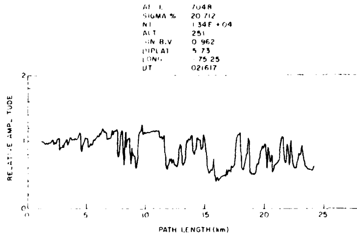
Fig. 6. A 3-s sample of high resolution RPA data of relative amplitude obtained on orbit 7048 indicating the presence of steep spatial gradients of ion concentration before the satellite entered a deep bite-out region in the early phase of irregularity generation. The satellite location maps along the earth's magnetic field lines to a 3-m plume structure over Jicamarca. The irregularity amplitude, (SIGMA%), the ion concentration (NI) at the beginning of the data interval, the satellite altitude (ALT), the sine of the angle between the magnetic field (B) and the satellite velocity (V) vectors, the dip latitude (DIPLAT), geographic longitude (LONG), and the universal time (UT) are indicated in the figure.
