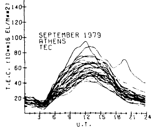
Fig. 5. Monthly overplot of TEC vs UT as Athens, Greece for June, 1979. Fig. 6. Same as Fig. 5 for September, 1979.
