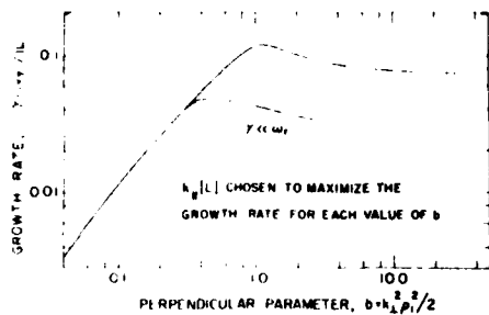
Fig. 14. Growth rate \gamma as function of the parameter b . The curve labeled \gamma(\omega) is obtained from the 'small growth rate' expression, while the unlabeled curve is obtained from the 'generalized' expressions [after Costa and Kelley , 1978b]
