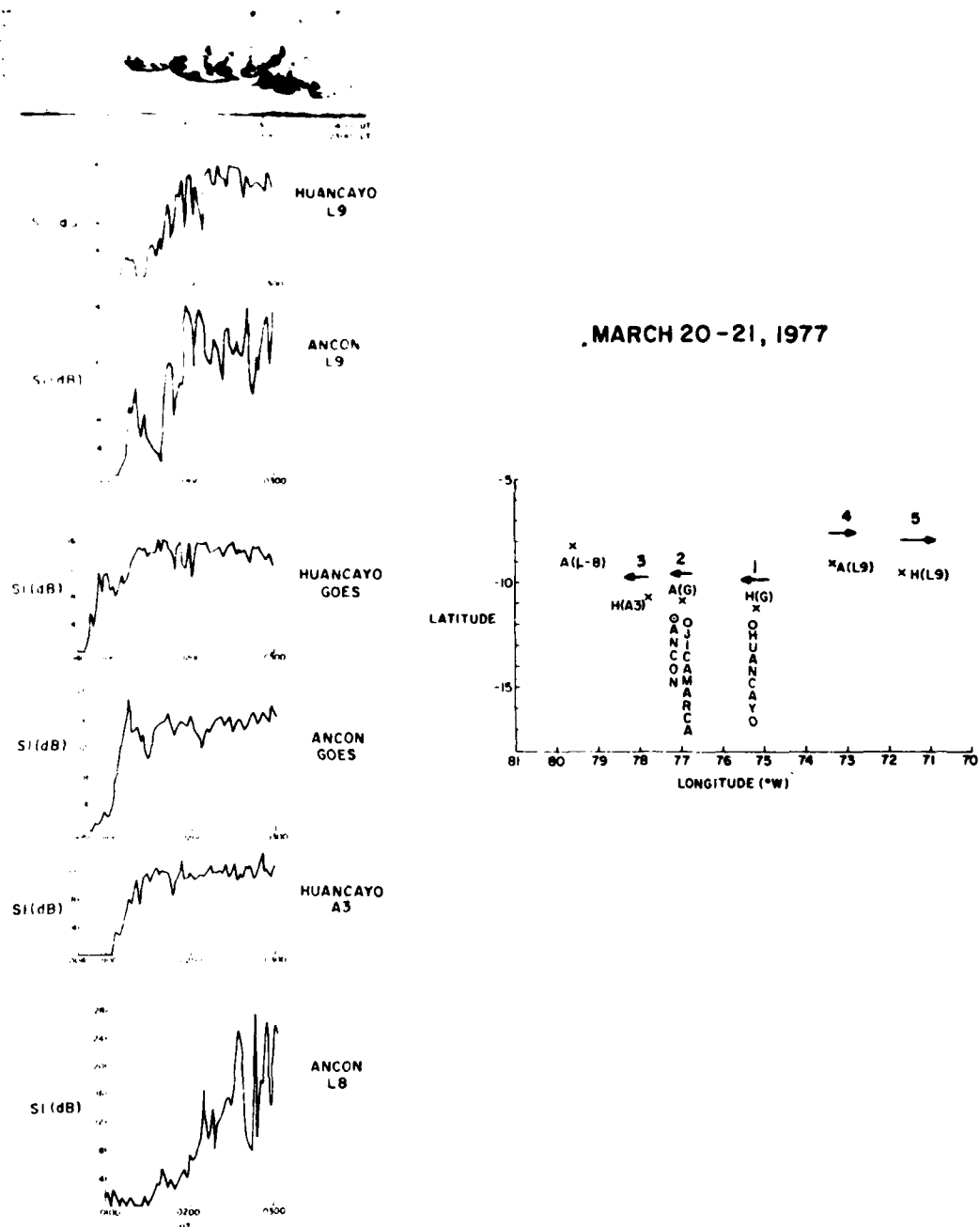
Fig. 3. Backscatter and scintillation data recorded on March 20-21, 1977, of several satellites observed from Ancon and Huancayo, Peru. Through the use of arrows and the numerical order of commencements on the accompanying map, one can see the westward development of the irregularity patch (over a longitude range 75°-78°W), the end of the westward motion, and finally the eastward motion across the L-9 paths. The ground positions of the sites and the 400-km sub-ionospheric positions are illustrated as in Figure 2.
