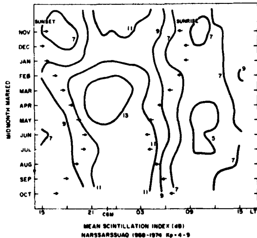
Fig. 3. Same as for Figure 2, except for disturbed magnetic conditions ( K_p = 4-9 ).
