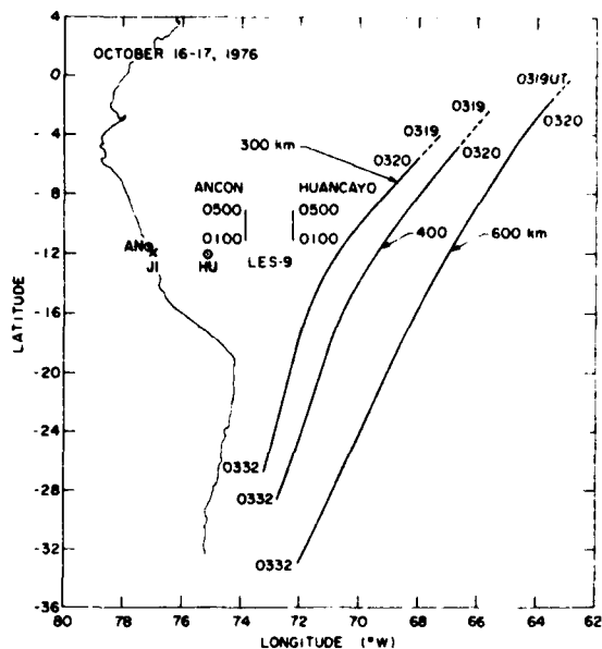
Fig. 1. Geometry of radar backscatter and scintillation measurements on October 16-17, 1976. The ground locations of Jicamarca (JI), Ancon (AN), and Huancayo (HU) are indicated. The subionospheric locations (400 km) of Les 9 observations from Ancon and Huancayo between 0100 and 0500 UT are shown. The subionospheric tracks of the Wideband satellite between 0319 and 0332 UT corresponding to 300, 400, and 600 km are also shown. The western coastline of South America is indicated for reference purposes.
