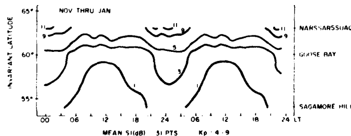
Fig. 15. Same as in Figure 14, except for \sim 31 values for each hourly data point for disturbed magnetic conditions ( K_p = 4.9 )
