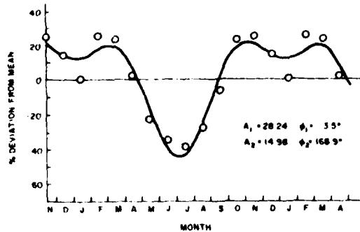
Fig. 12. Seasonal variation of 136-MHz scintillation from ATS 3 at Legon, Ghana, during the period September 1971 to December 1975. Note that the annual component (with a minimum in the June solstice) has twice the amplitude of the semiannual component [after Koster, 1976].
