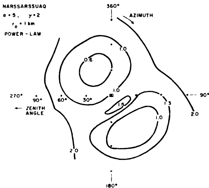
Fig. 7. Plot of correction factors for viewing a 1100-km orbiting satellite from Narsarsuaq under assumptions of elliptical column irregularity model and a power law irregularity power spectrum.
