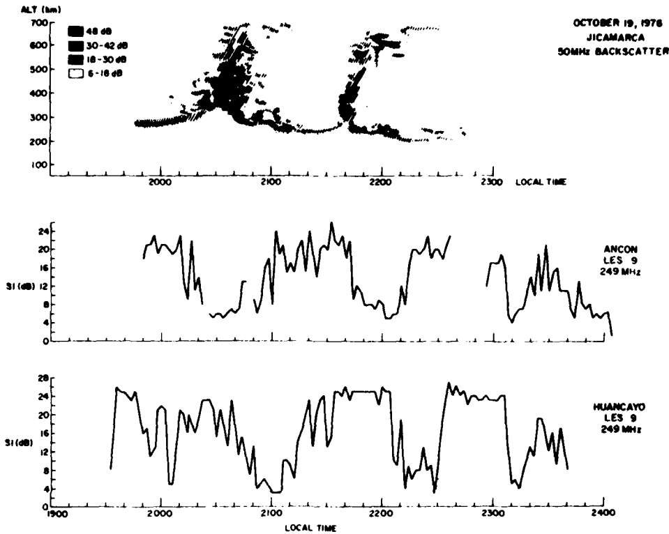
Fig. 4. Temporal variation of the 50-MHz radar backscatter observed at Jicamarca and scintillation index, SI (dB), of the 249-MHz transmissions from the Les 9 satellite recorded at Ancon and Huancayo on October 19-20, 1976 [after Basu and Aarons, 1977].
