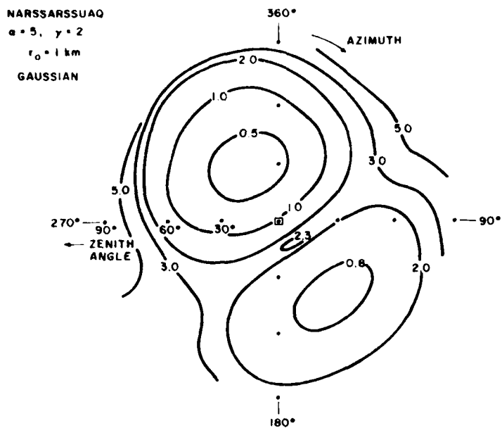
Fig. 6. Plot of correction factors for viewing a 1100-km orbiting satellite from Narsarsuaq under assumptions of elliptical column irregularity model and a Gaussian irregularity power spectrum.
