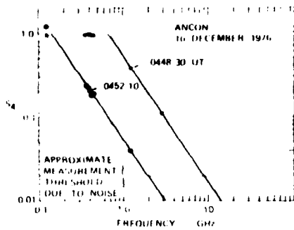
Fig. 11. Frequency dependence of intensity-scintillation index during two 20-s periods of the Ancon Wideband pass on December 16, 1976, compared with an f^{-3.5} dependence [after Fremouw et al. , 1978].
