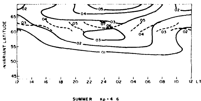
Fig. 9. Comparison of Wand and Evans 400-MHz summer data for the disturbed magnetic case (solid curves) with Narssarssuaq and Goose Bay model data (dashed curves) corrected for the ATS 3 intersection point and converted to 400 MHz.
