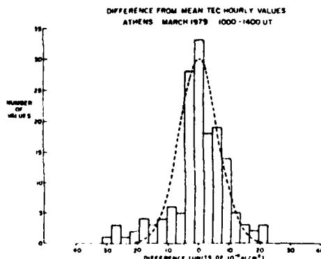
Fig. 9. Distribution of differences from mean hourly TEC values for Athens, Greece, March, 1979, 1000-1400 UT. Dashed curve is a Gaussian curve of standard deviation 9.0.
