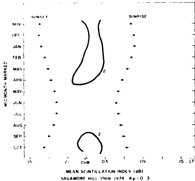
Fig. 6 Contours of monthly mean scintillation index in decibels at 137 MHz as a function of local time for quiet magnetic conditions ( K_p = 0-3 ) obtained at Sagamore Hill with ATS 3 during 1968-1974.
