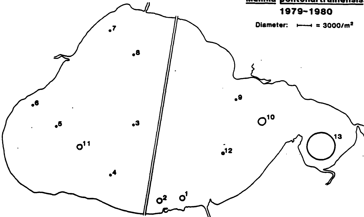
Figure 37. Annual mean Mulinia pontchartrainensis abundance for each sampling station in Lake Pontchartrain. Upper map, 1978-1979; lower map, 1979-1980.
