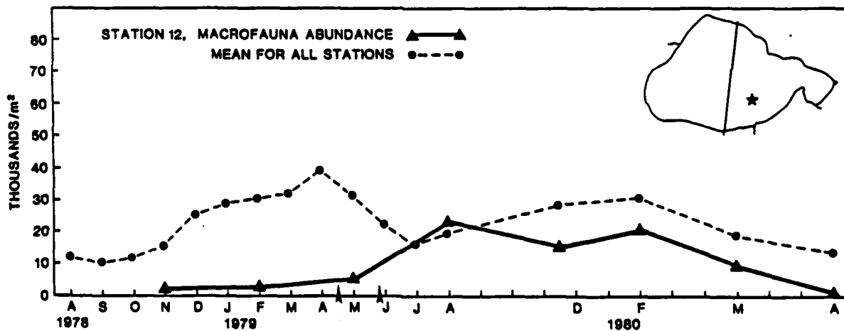
Figure 31. Macrofauna Abundance, Station 12.
