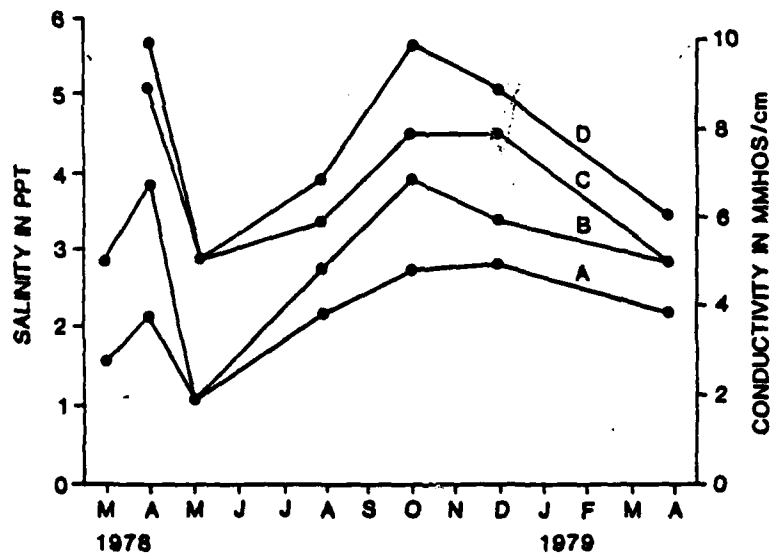
Figure 8. Lake Pontchartrain responds as a whole to seasonal salinity fluctuations despite salinity differences between the four regions. (data from Swenson 1980a)
