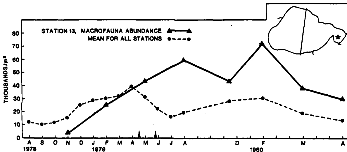
Figure 33. Macrofauna Abundance, Station 13.
