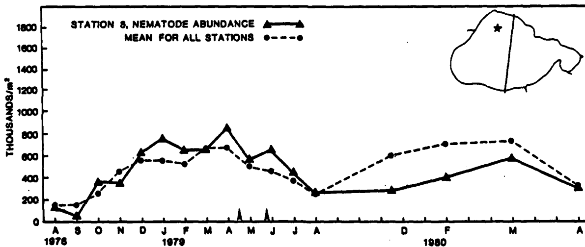
Figure 24. Nematode Abundance, Station 8.
