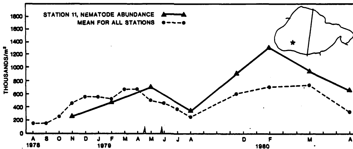
Figure 30. Nematode Abundance, Station 11.
