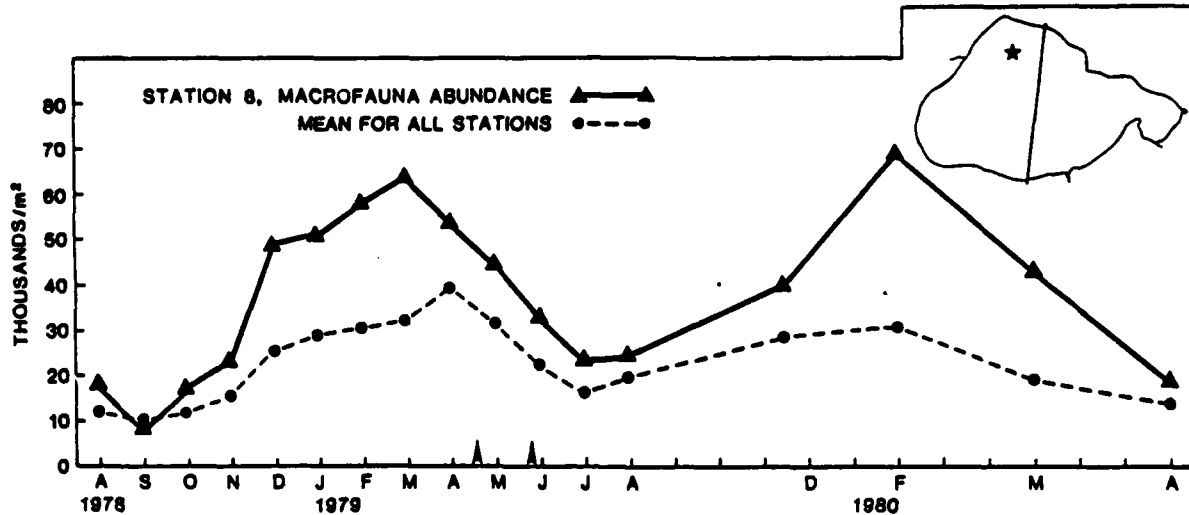
Figure 23. Macrofauna Abundance, Station 8.
