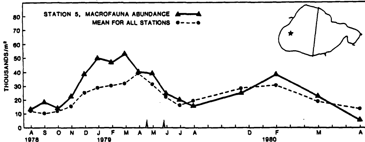
Figure 17. Macrofauna Abundance, Station 5.
