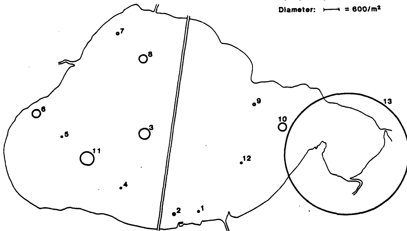
Figure 40. Annual mean amphipod abundance for each sampling station in Lake Pontchartrain. Upper map, 1978-1979; lower map, 1979-1980.
