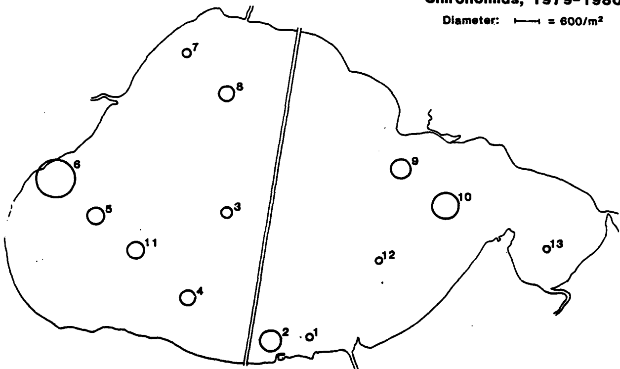
Figure 38. Annual mean chironomid abundance for each sampling station in Lake Pontchartrain. Upper map, 1978-1979; lower map, 1979-1980.
