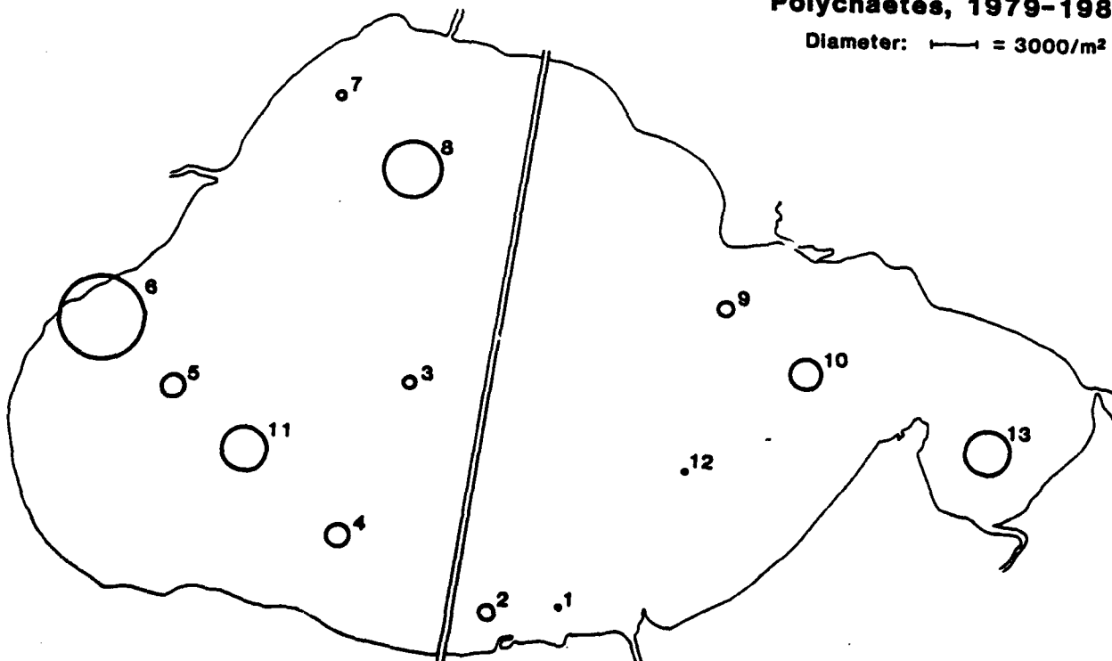
Figure 39. Annual mean polychaete abundance for each sampling station in Lake Pontchartrain. Upper map, 1978-1979; lower map, 1979-1980.
