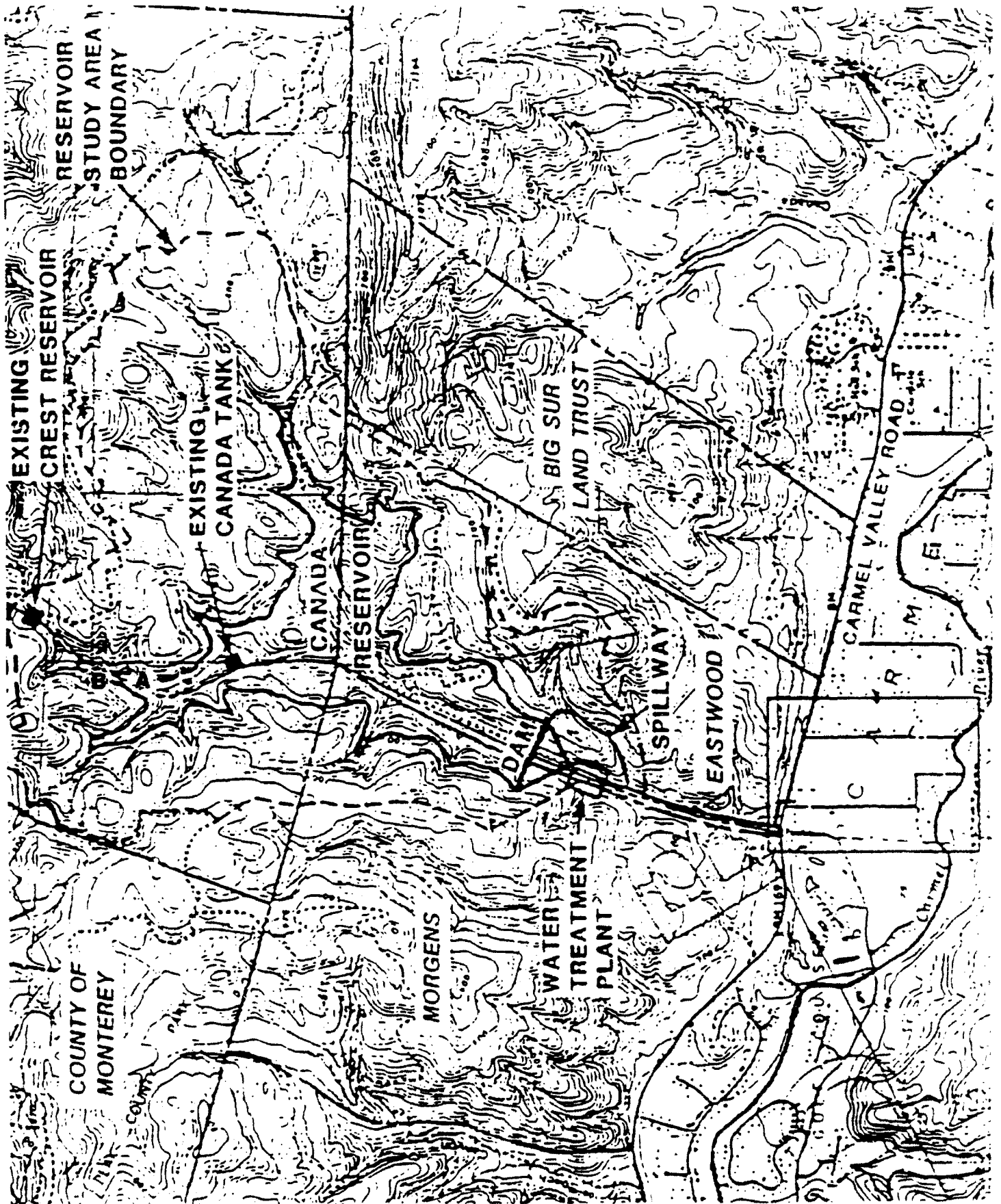
FIGURE 4 SURVEY RESULTS
