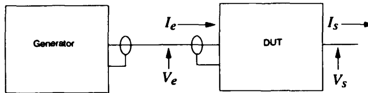
Figure 44. Power PPD test setup.
