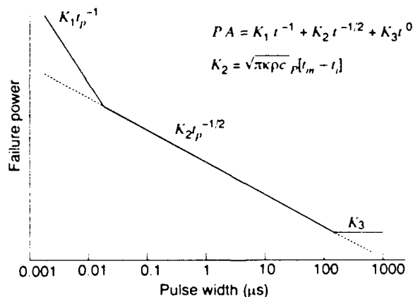
Figure 31. Wunsch factor.
