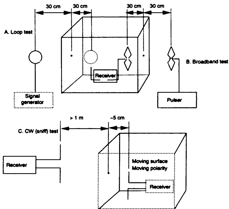
Figure 36. Antenna positions.
