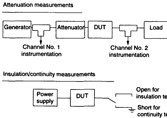
Figure 40. Voltage test setup.
