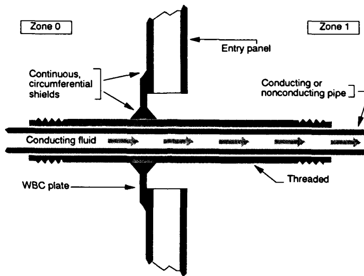
Figure 23. Incorrect waveguide.
