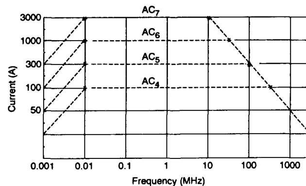
Figure 13. External current range.
