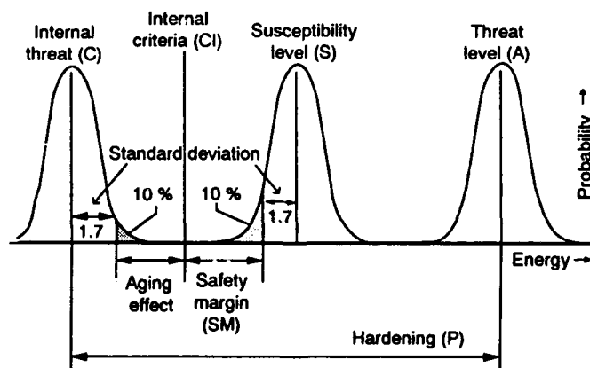
Figure 10. Statistical guidelines.
