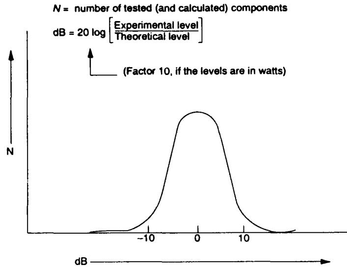
Figure 32. Statistical error.
