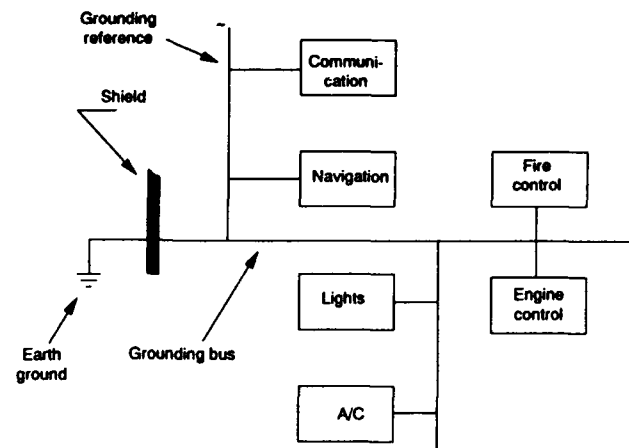
Figure 3. Grounding connections.
