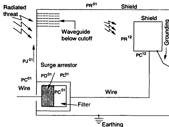
Figure 11. Protection methods.
