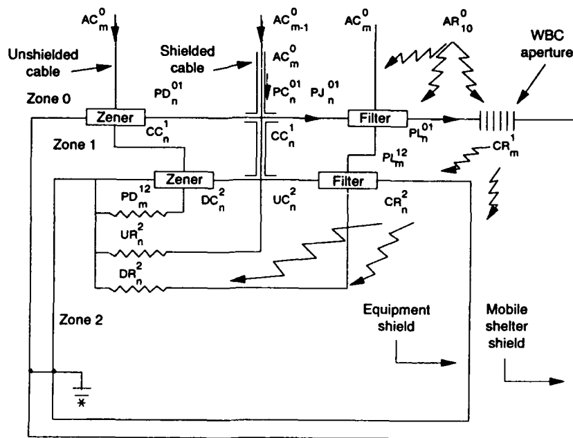
Figure 1. Guideline terms.
