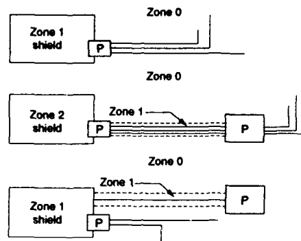
Figure 14. Cable protection.
