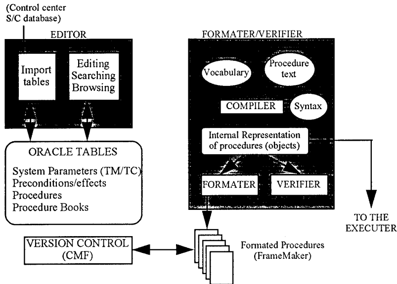
FIGURE 4/2 - OPSMAKER ARCHITECTURE
