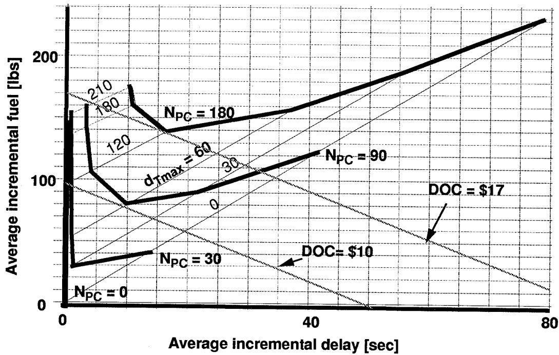
Figure 9.- Carpet plot
