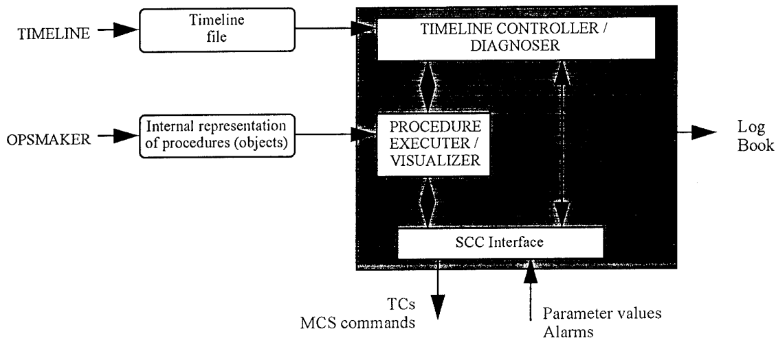
FIGURE 6.1 - OPSEXCUTER ARCHITECTURE
