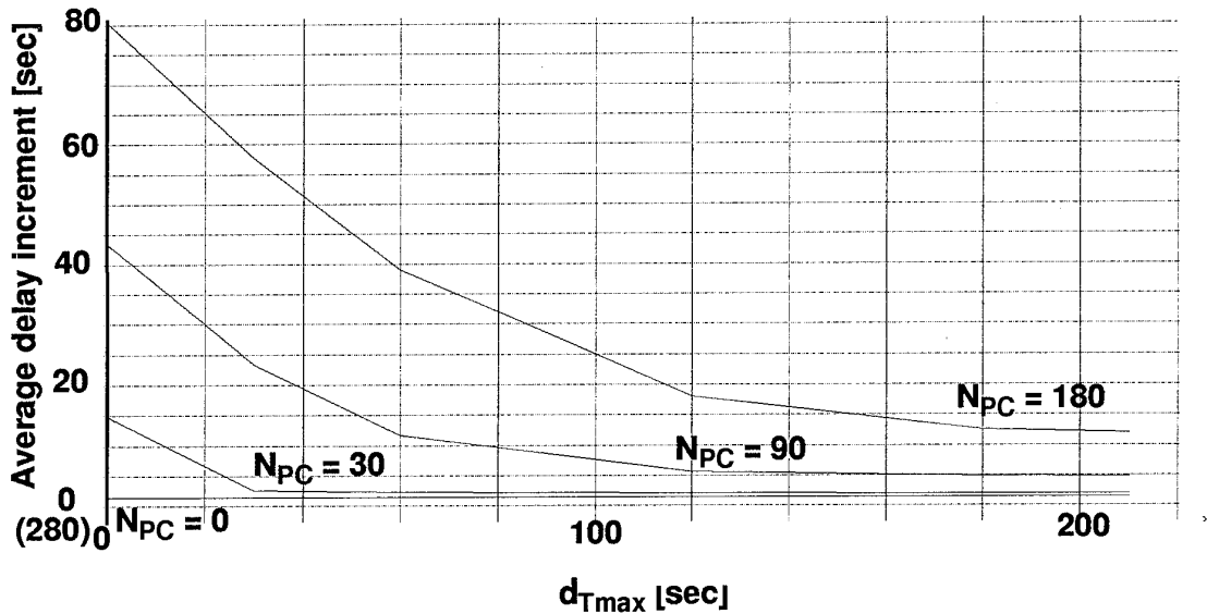
Figure 7.- Average delay increment for 36 aircraft/hour for a single runway vs d_{Tmax}
