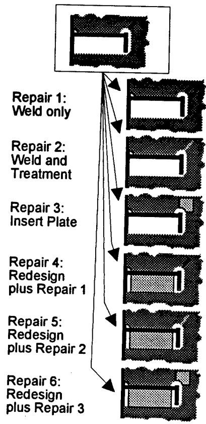
Figure 3.2: Six repair alternatives on a fatigue crack in cutout radius.
