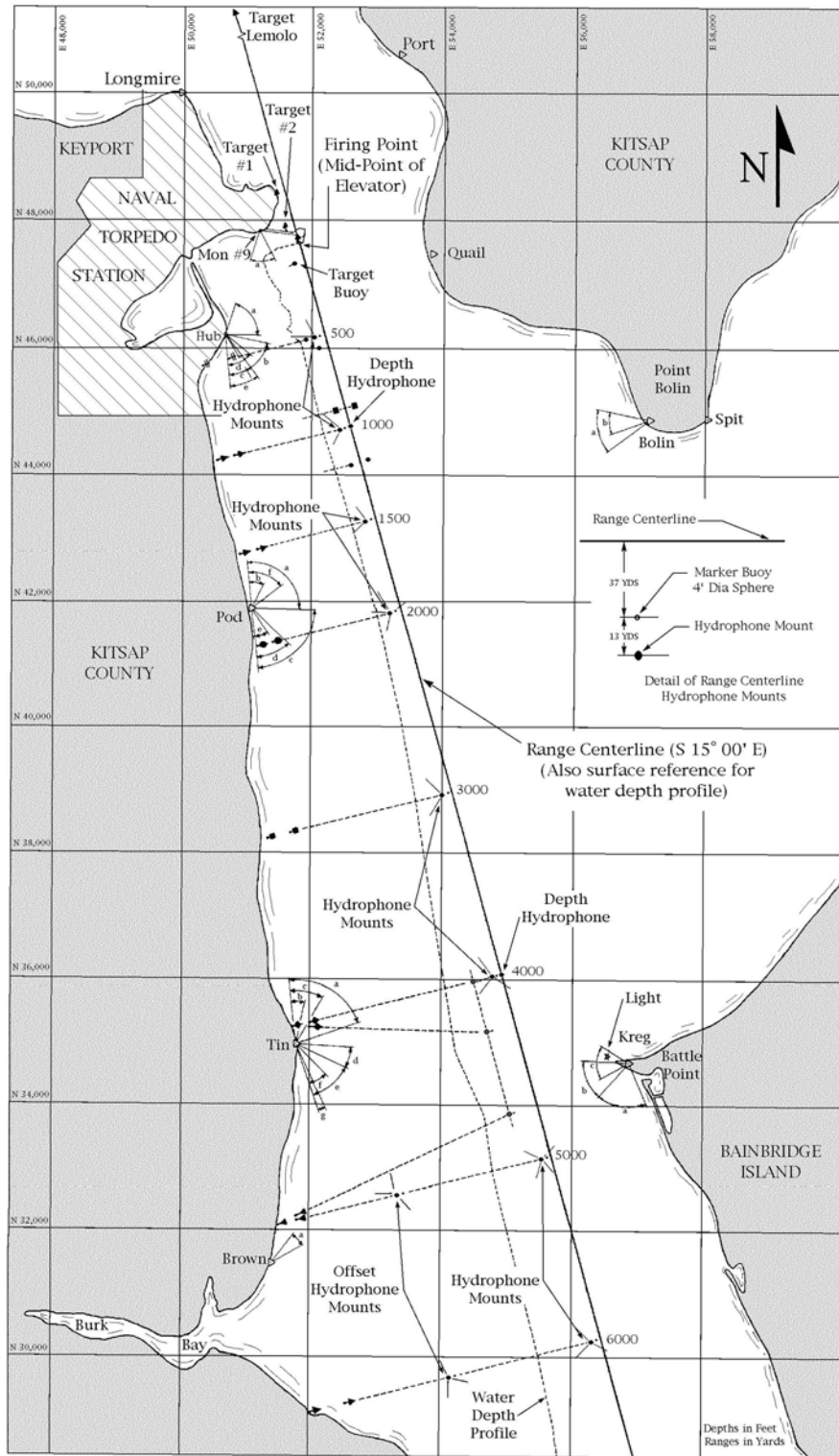
Keyport Acoustic Range Layout (Circa 1957)
