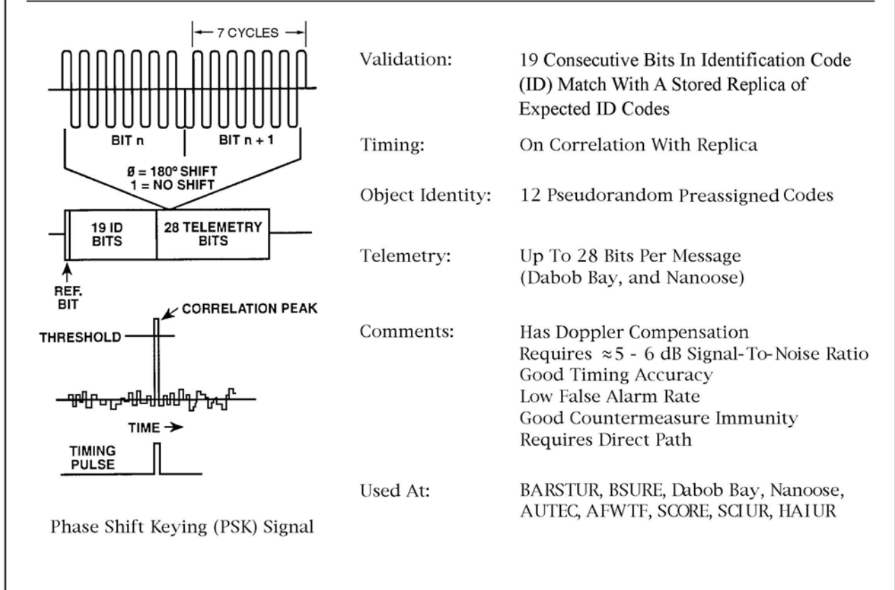
Tone Burst and Phase-Shift Keying (PSK) Signal Characteristics
