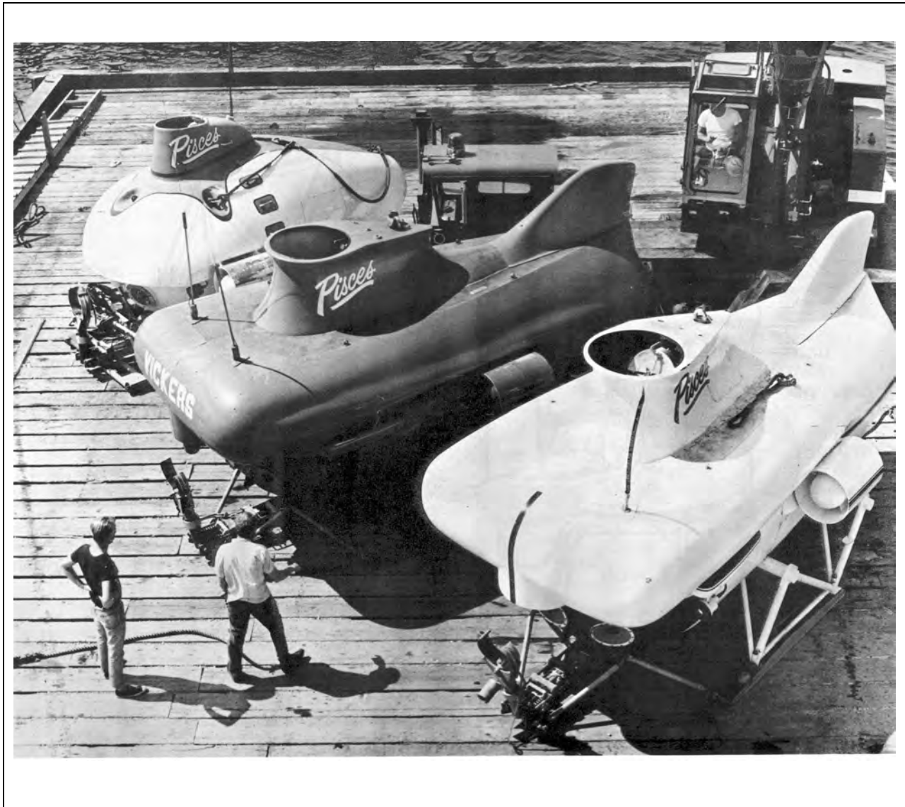
The Pisces Manned Submersible (Note the torpedo recovery clamps)
