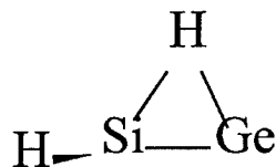
FIGURE 10. HSiHGe (C s ).
