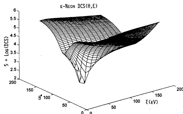
FIGURE 3. Differential cross section (DCS in atomic units) surface for e-neon system showing a minimum near ( 95^\circ, 65 eV).
