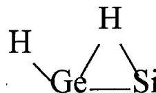
FIGURE 9. HGeHSi (C s ).
