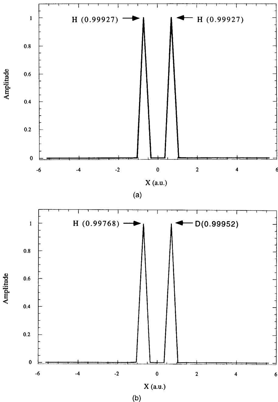
FIGURE 3. Nuclear density of (a) H_2 , (b) HD , and (c) D_2 (a.u.) using converged wave functions. The range of figures are from i = 48-80 . H and D represent the proton and deuteron, respectively. The numbers in a parentheses denote the maximum density.
