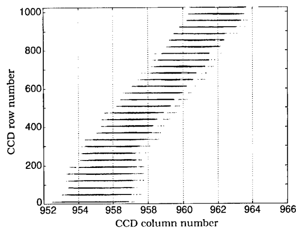
FIGURE 5. Timing comb pulses used to determine the time step per row (14.32 ns / row) and the CCD mounting error (a - 6 row error at the columns corresponding to the \text{Re}_2\text{Cl}_8^{2-} absorption).
