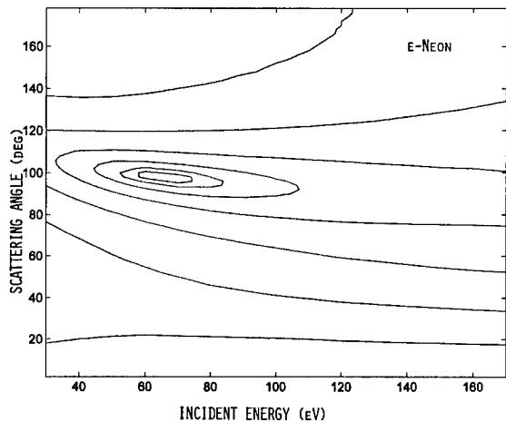
FIGURE 4. Contour plot corresponding to Figure 3 showing the approximate minimum of the surface at (95°, 65 eV).
