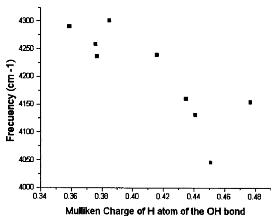
FIGURE 2. Relationship between the HF/6-31 + G(d, p) calculated frequency of the OH vibrational mode and the HF/6-31 + G(d, p) Mulliken population of the H atom of the OH bonds in the zeolite cluster acid sites.
