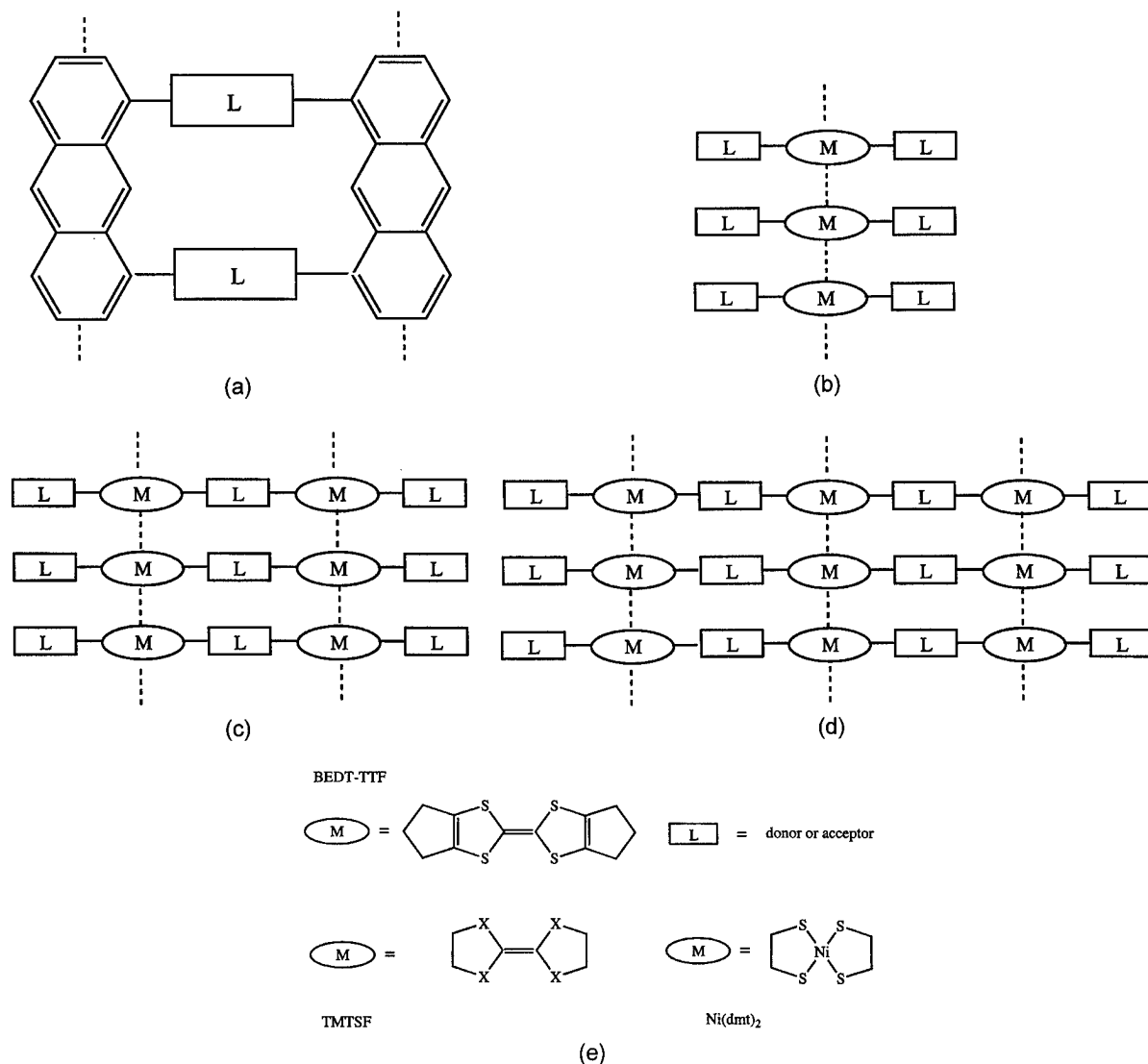
FIGURE 7. Some possible models of polymer network and crystal systems for the superconductor.
