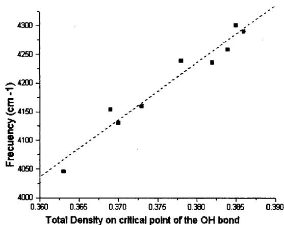
FIGURE 1. Relationship between the HF/6-31 + G(d, p) calculated frequency of the OH vibrational mode and the HF/6-31 + G(d, p) total density, calculated at the position of the critical point of OH bonds in the zeolite cluster acid sites. Linear correlation coefficient is r^2 = 0.98 .
