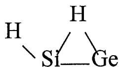
FIGURE 8. HSiHGe (C s ).
