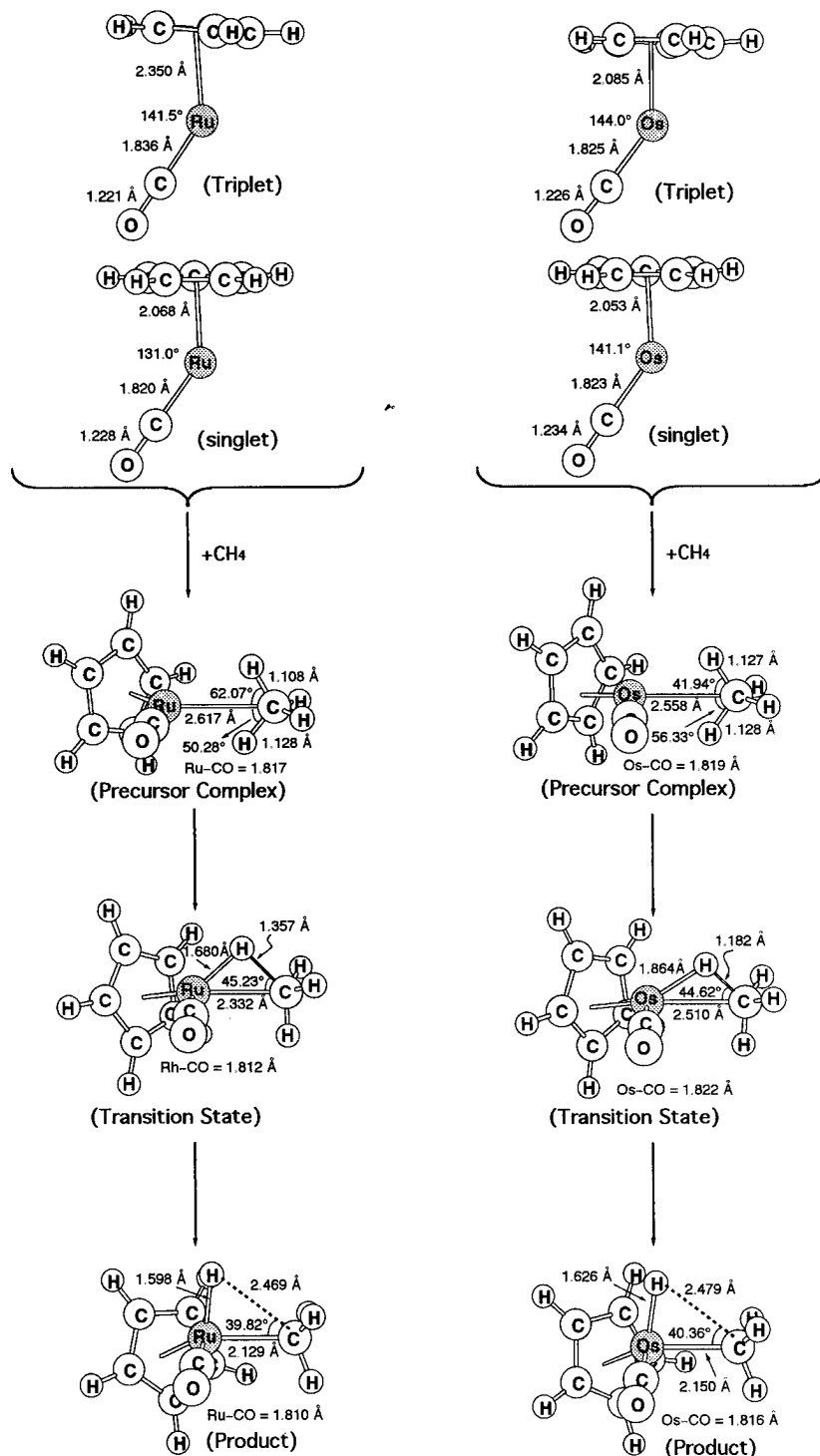
FIGURE 3. Optimized structures at the B3LYP / LANL2DZ level for the [CpRu(CO)] - and {CpOs(CO)} - systems.
