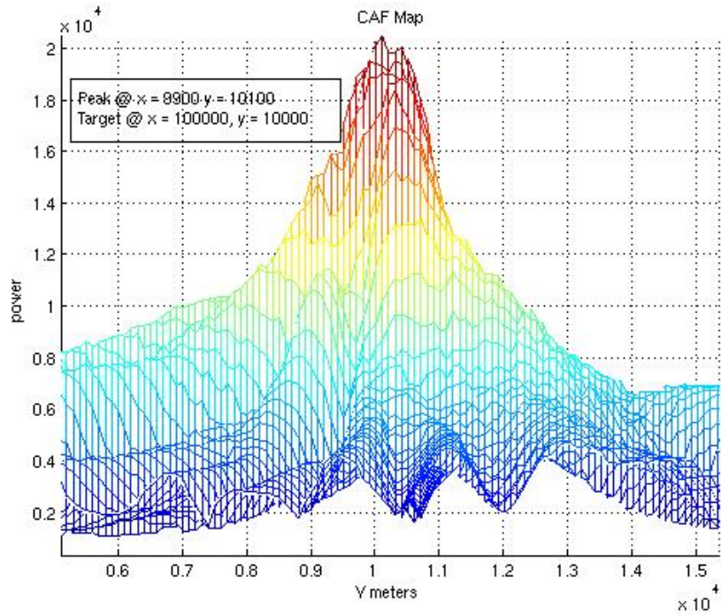
Figure 5-31: Y-Z CAF-Map
