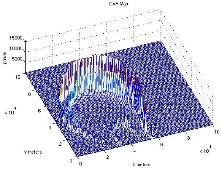
Figure 5-37: CAF-Map from collection pair at P1 = [35e3,0], P2 = [45e3,5e3] meters
