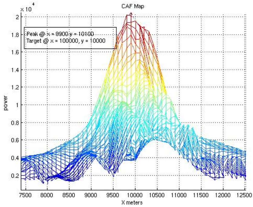
Figure 5-30: X-Z CAF-Map
